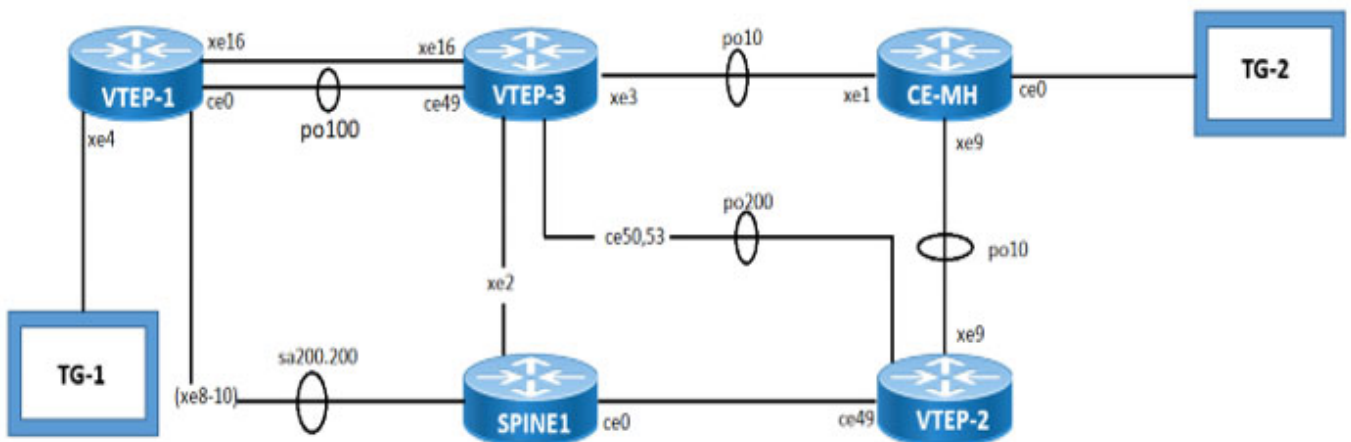
Figure 3-11: Multi-homed VxLAN Eline xConnect topology
