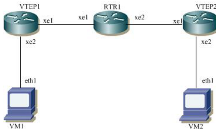
Figure 1-3: VxLAN unicast
