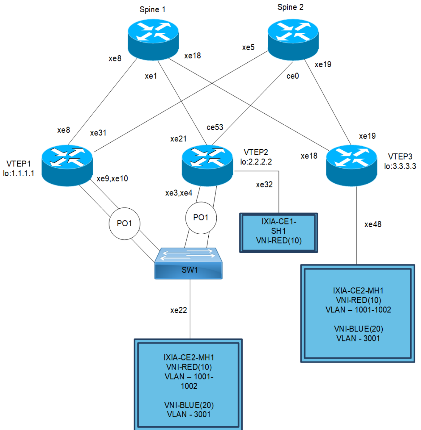
Figure 2-6: VxLAN-Multihoming
