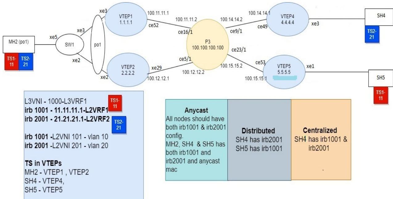
Figure 2-9: VxLAN_EVPN_IRB
