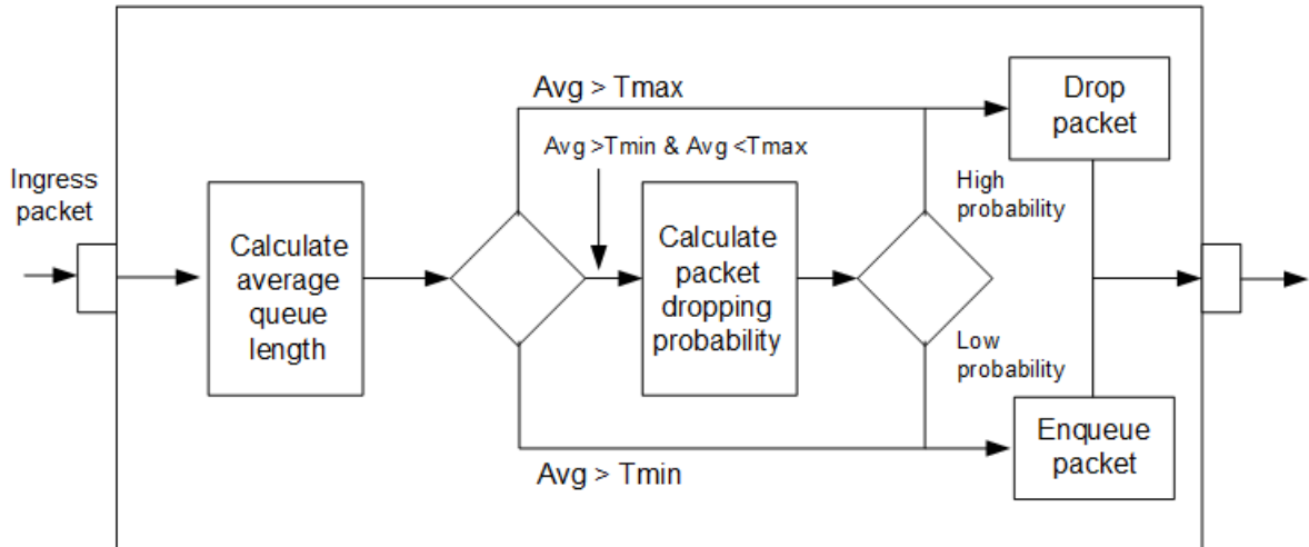
Figure 13-1: Weighted random early discard flow algorithm
