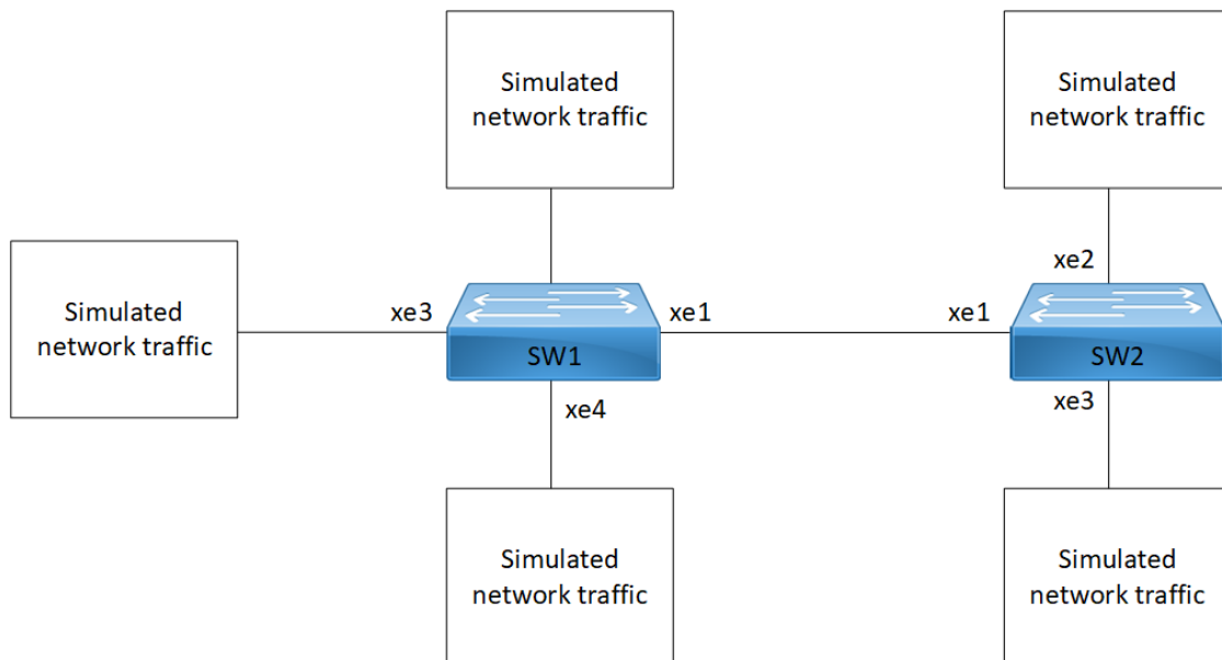
Figure 18-39: PVLAN configuration
