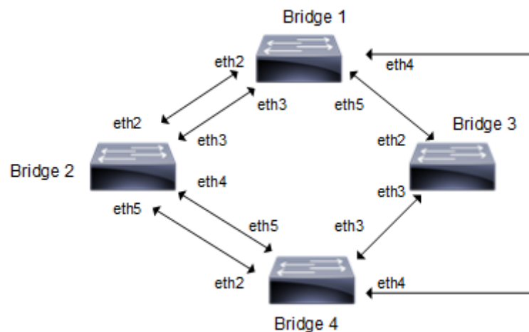
Figure 4-12: STP Topology
