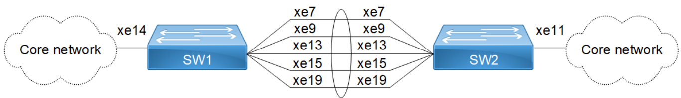
Figure 12-27: Port-Channel weight with dynamic LAG
