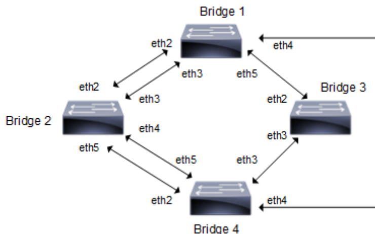
Figure 6-14: MSTP Topology
