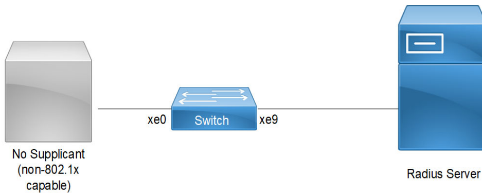
Figure 25-46: MAB Topology
