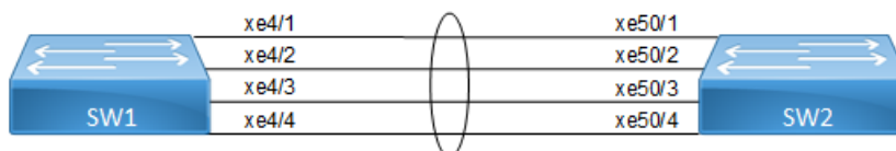
Figure 12-24: LAG minimum bandwidth
