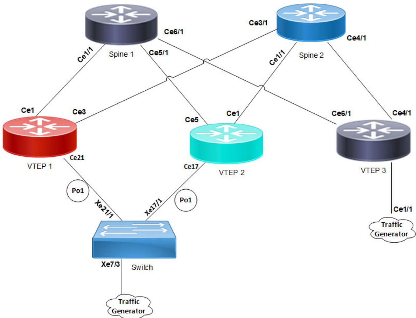
Figure 22-42: L2CP tunneling for VXLAN
