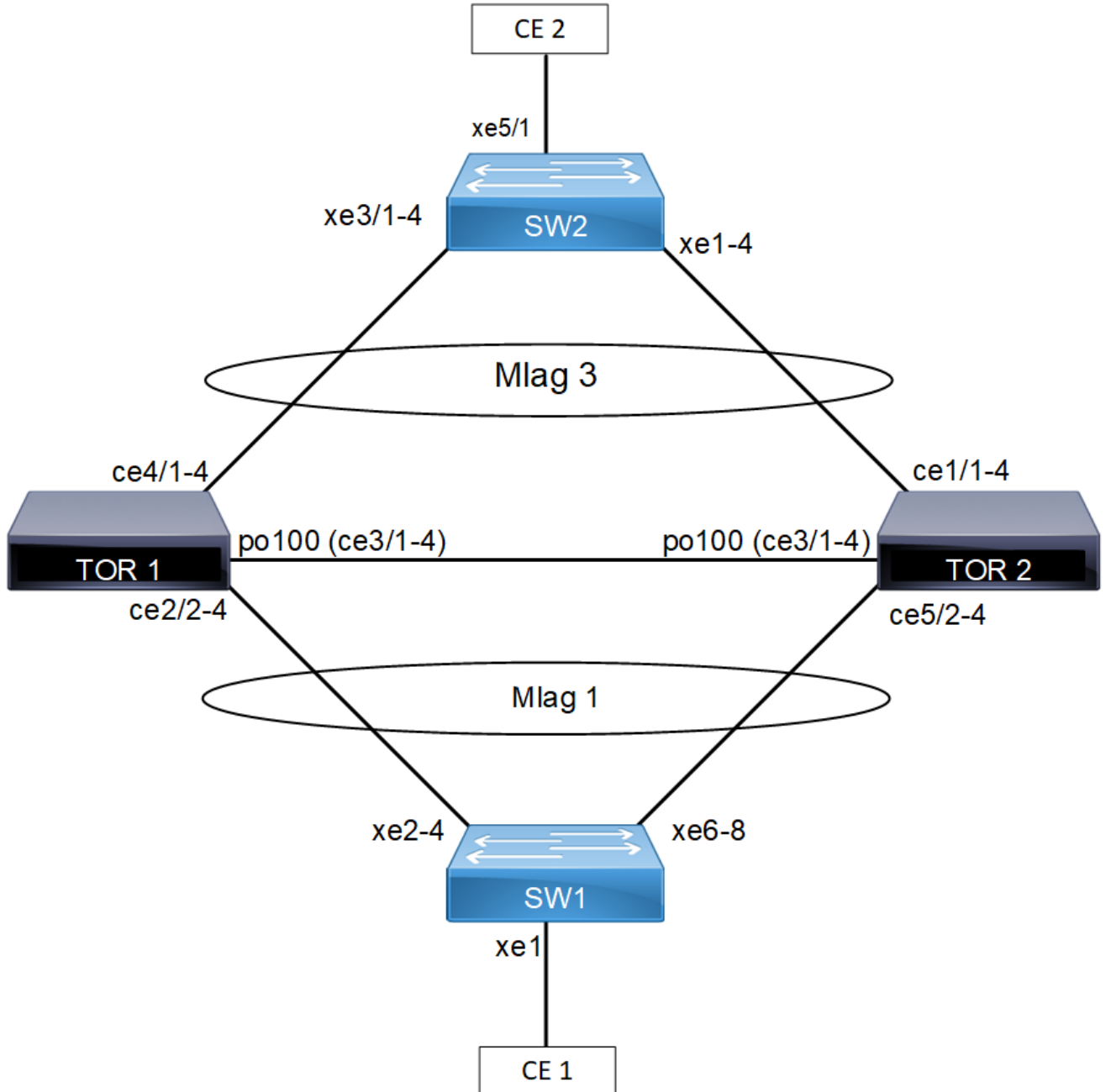
Figure 12-25: MLAG topology
