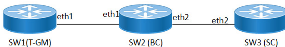
SMPTE PTP Configuration Topology
