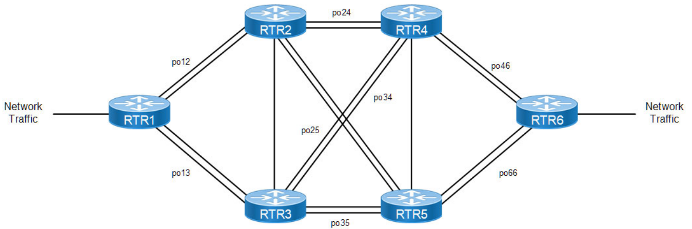
Figure 18-3: Simple Topology
