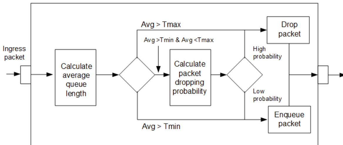
Figure 13-1: Weighted random early discard flow algorithm
