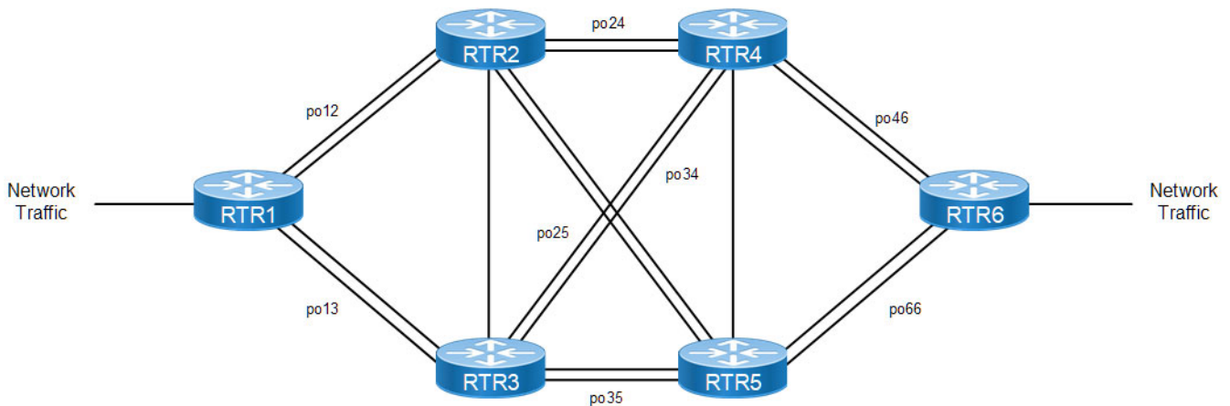
Figure 18-2: Simple Topology
