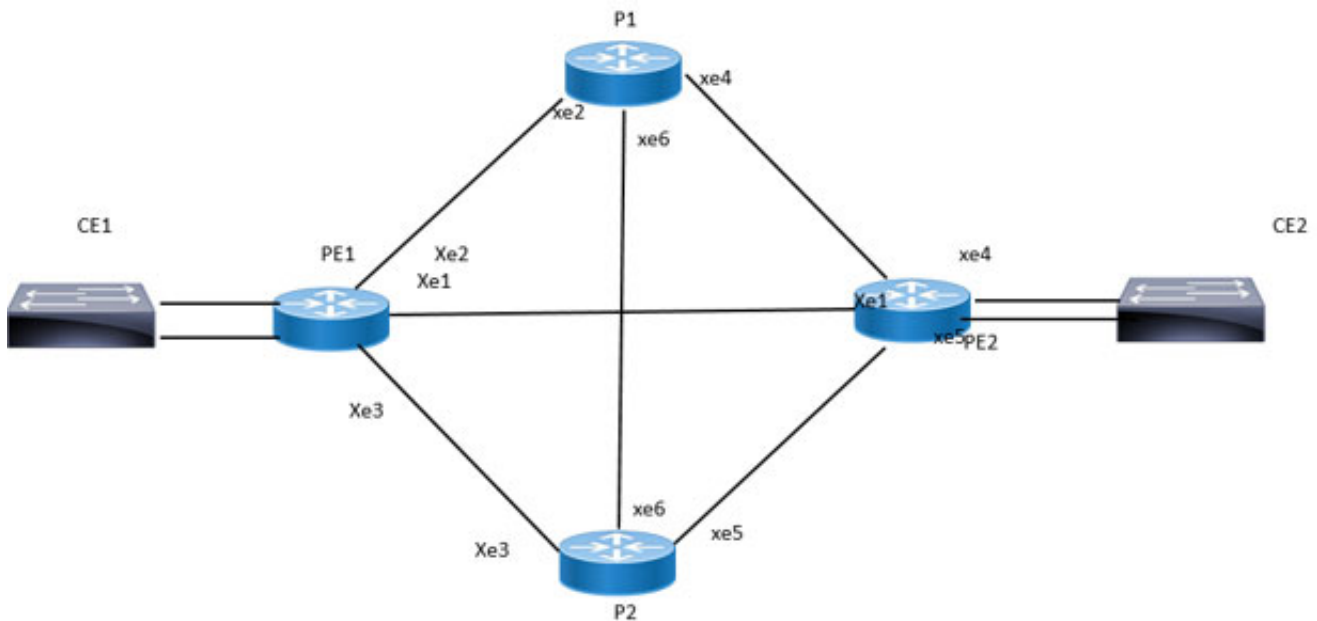
Figure 3-14: Figure 8-15: VPLS Mesh Peers split horizon
