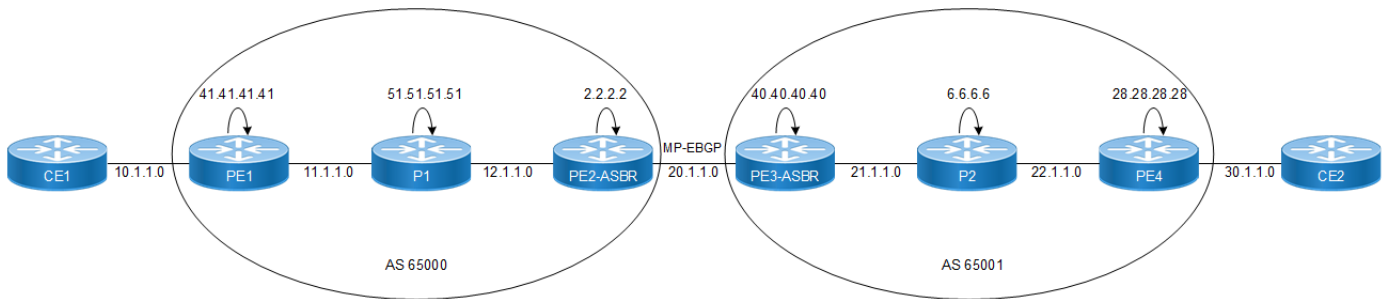
Figure 14-5: InterAS-VPN Option-C without RR
