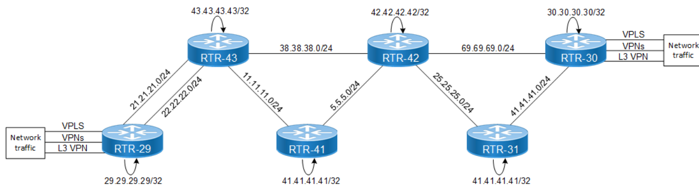
Figure 1-17: Topology Example for Fast Reroute
