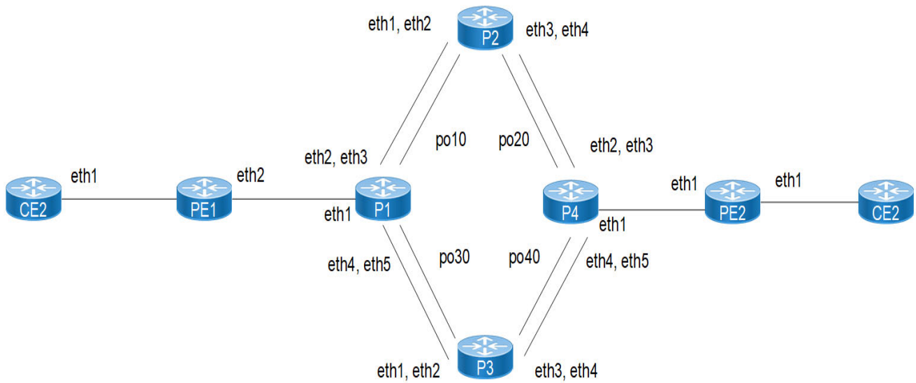
Figure 1-10: L2VPN configuration topology
