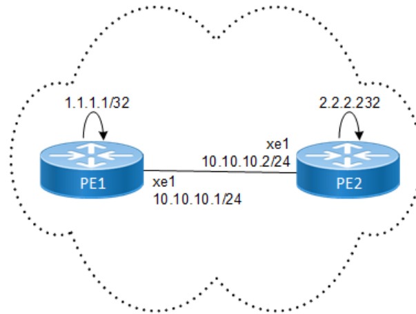
Figure 1-34: LDP Session Topology
