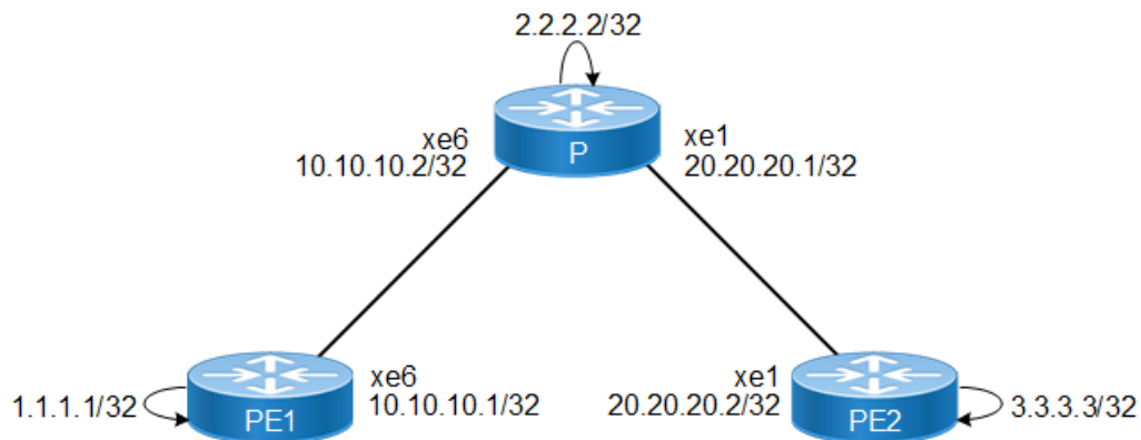
Figure 1-12: LDP Topology
