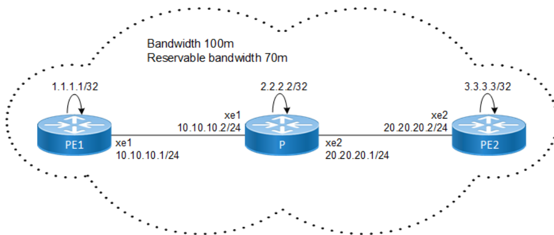
Figure 1-33: Topology for Targeted Session MD5
