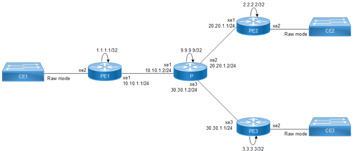
Figure 3-16: VPLS Tunnel-ID
