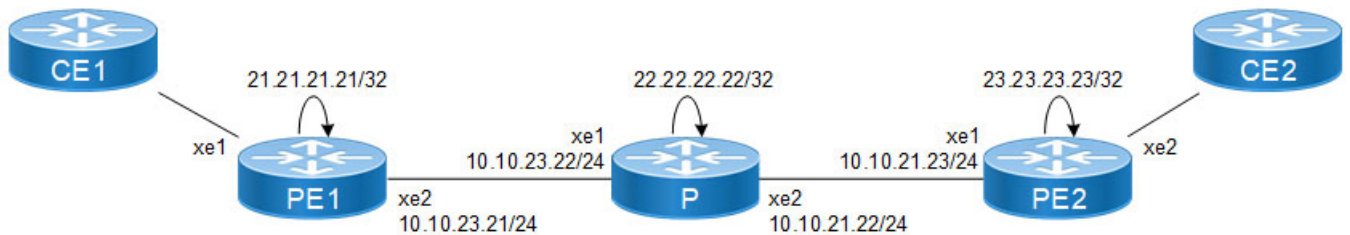
Figure 6-20: Static VPLS service mapping
