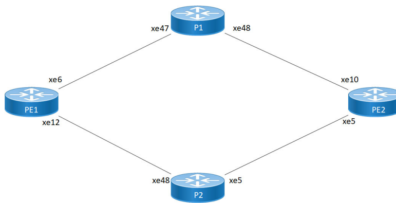
Figure 1-35: Basic LDP Topology
