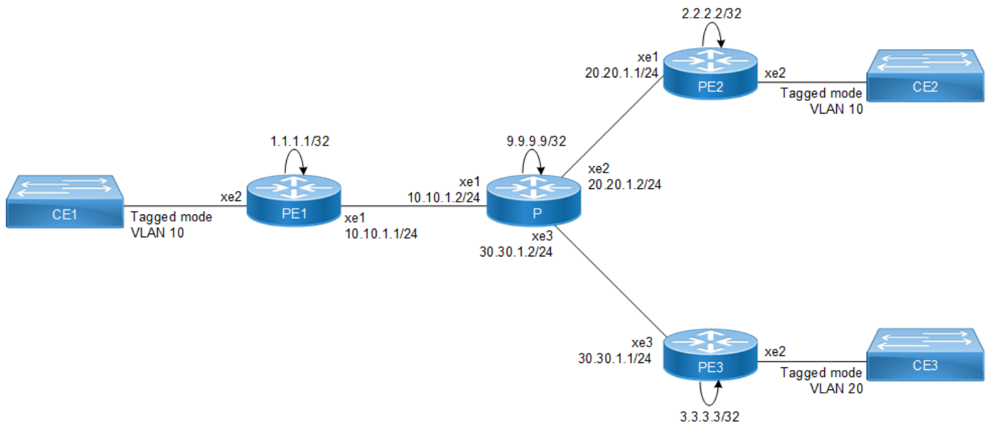
Figure 3-13: VPLS Mesh Peers Tagged Mode
