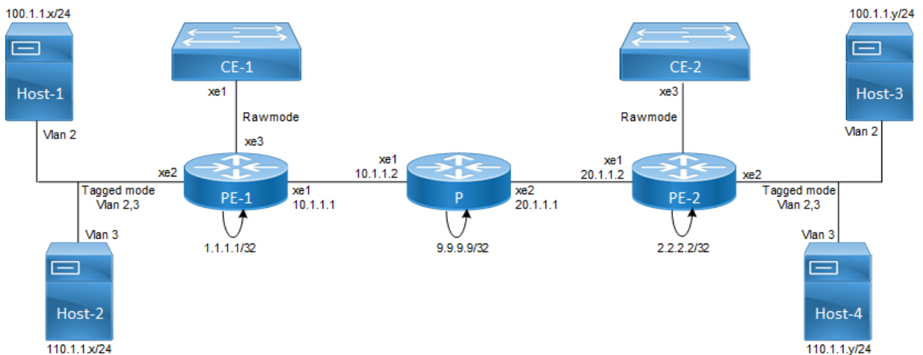
Figure 10-25: MPLS Layer 2 Virtual Circuit
