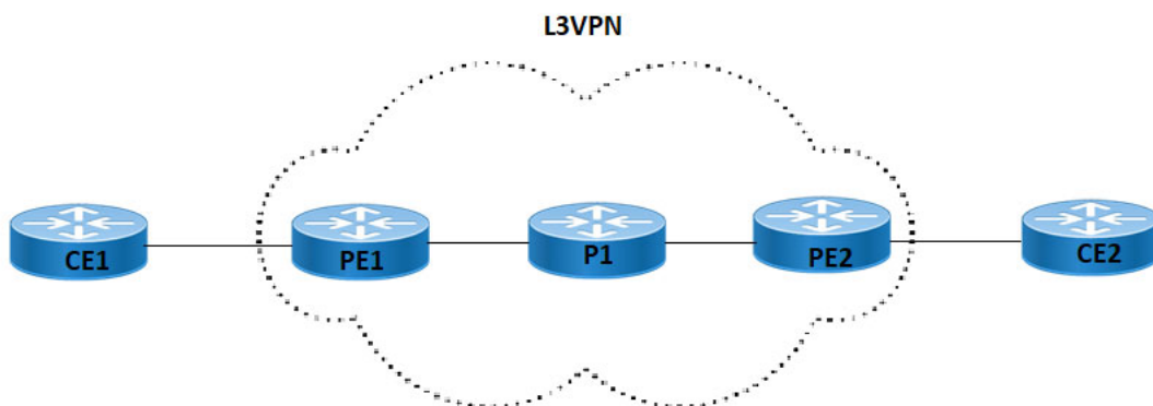
Figure 3-28: TWAMP over L3VPN Topology
