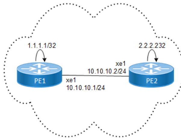
Figure 1-32: Topology for Direct Session MD5
