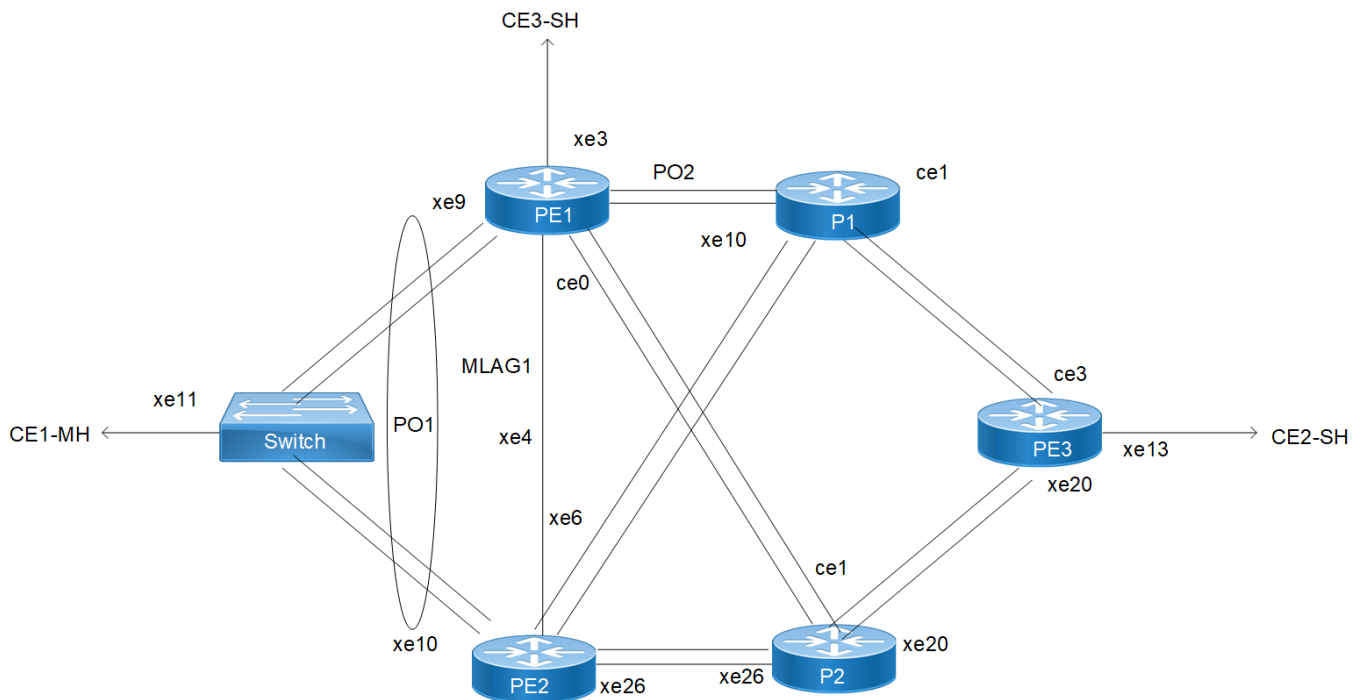
Figure 1-26: Topology diagram for L3VPN over EVPN MPLS
