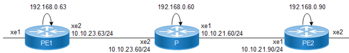
Figure 1-13: Basic Topology
