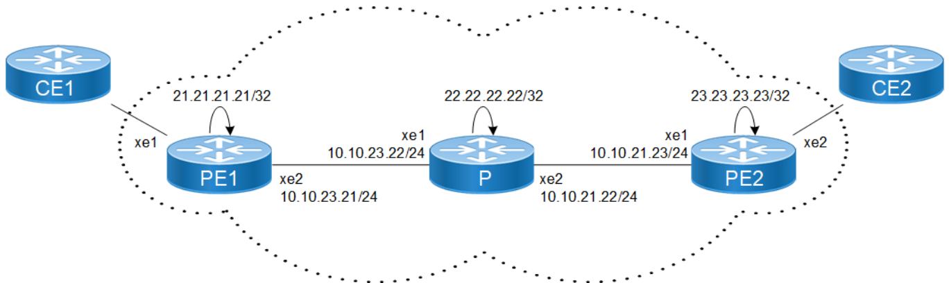
Figure 8-22: BGP-VPLS service mapping
