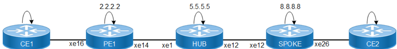
Figure 9-24: H-VPLS Configuration without Redundancy
