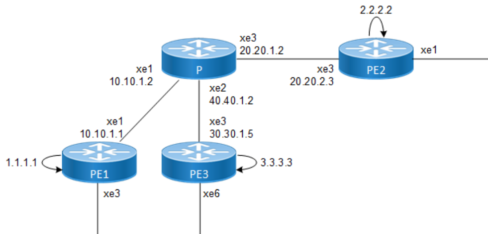
Figure 5-19: Sample Topology for VPLS with BGP Signaling
