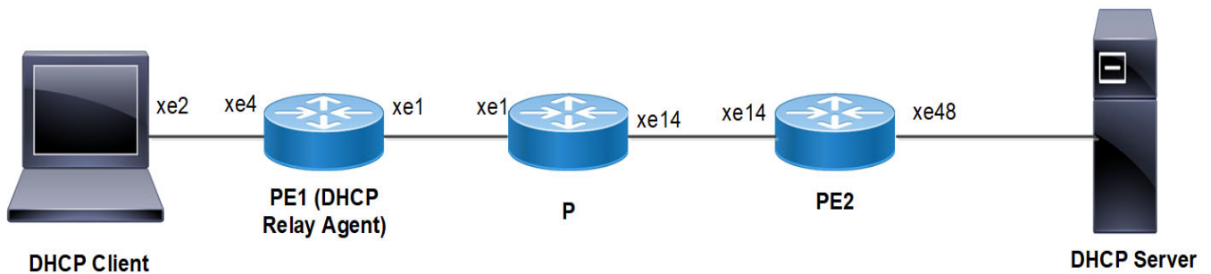
Figure 4-30: DHCP Relay Over L3 VPN Configuration
