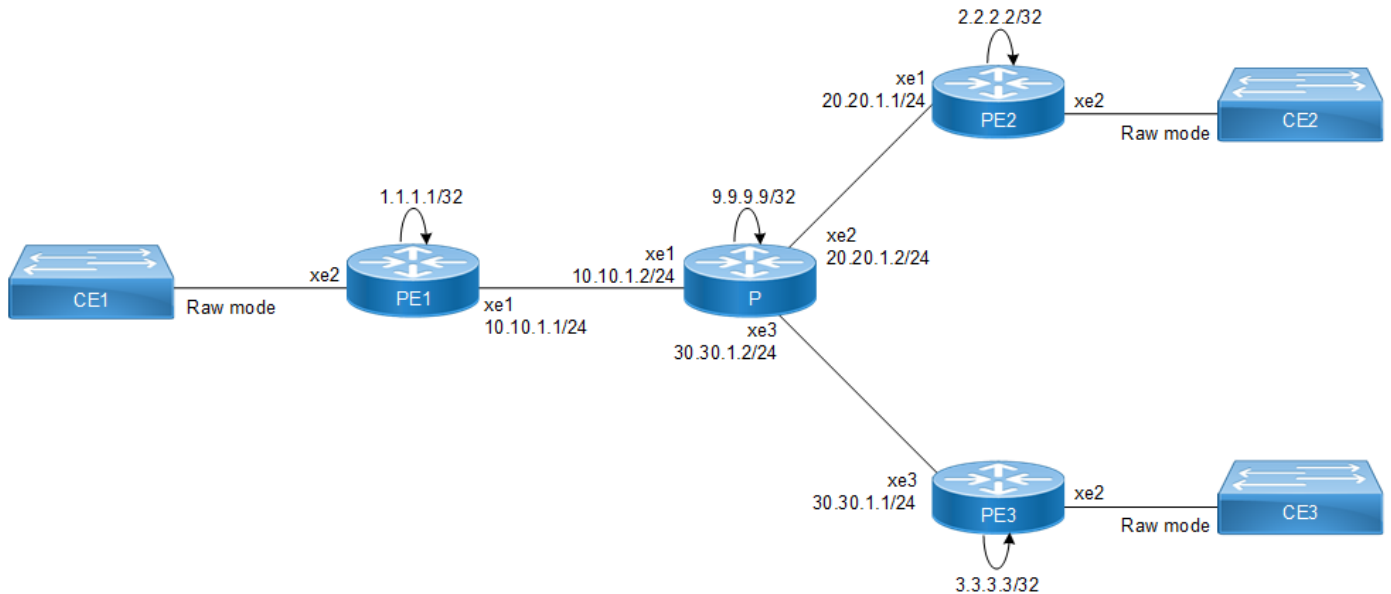
Figure 3-17: VPLS Tunnel-Name
