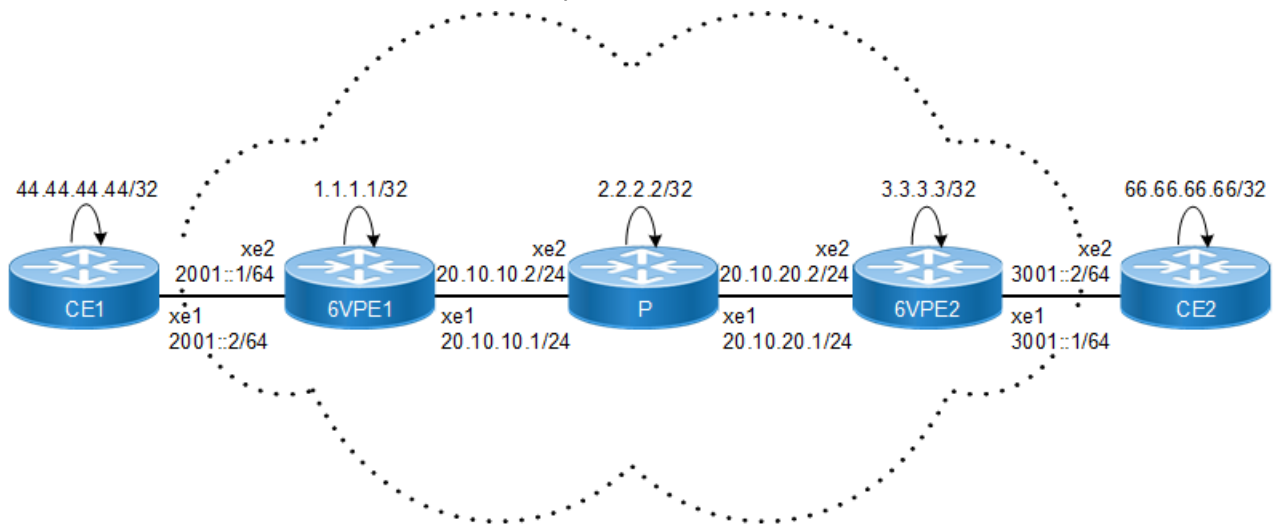
Figure 2-11: 6VPE Configuration
