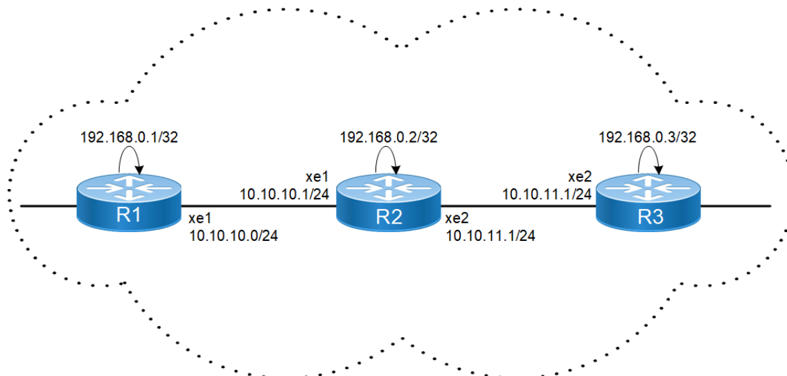
Figure 1-31: Basic LDP Topology
