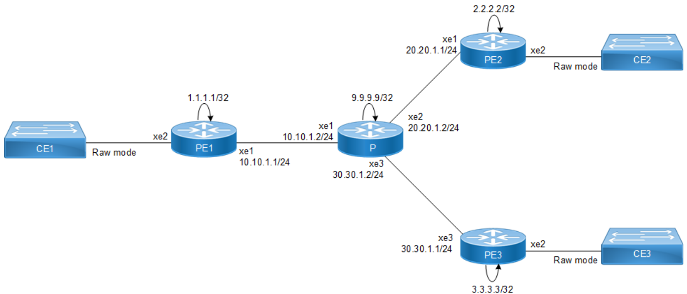
Figure 3-12: VPLS Mesh Peers Raw Mode
