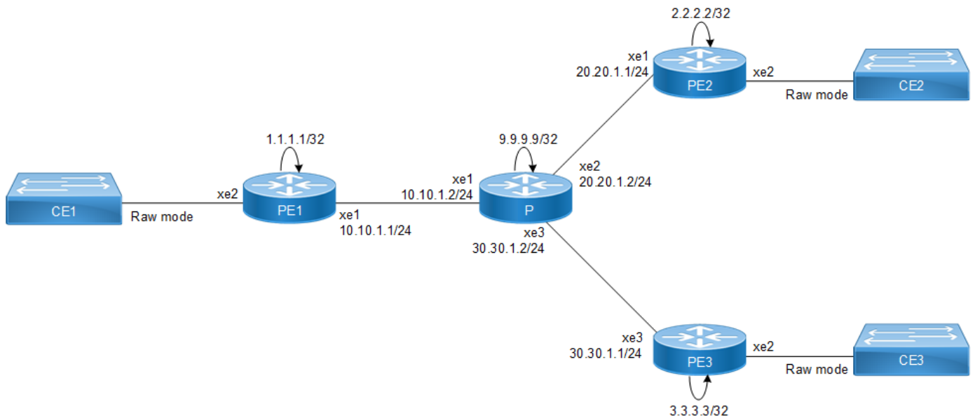
Figure 3-15: VPLS Per Peer VPLS Type Signaling
