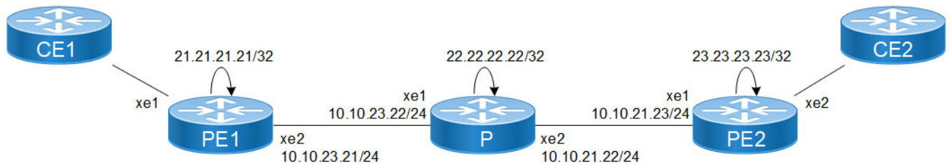
Figure 7-21: LDP-VPLS service mapping
