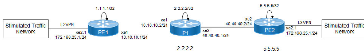
Figure 2-27: L3VPN GR Topology
