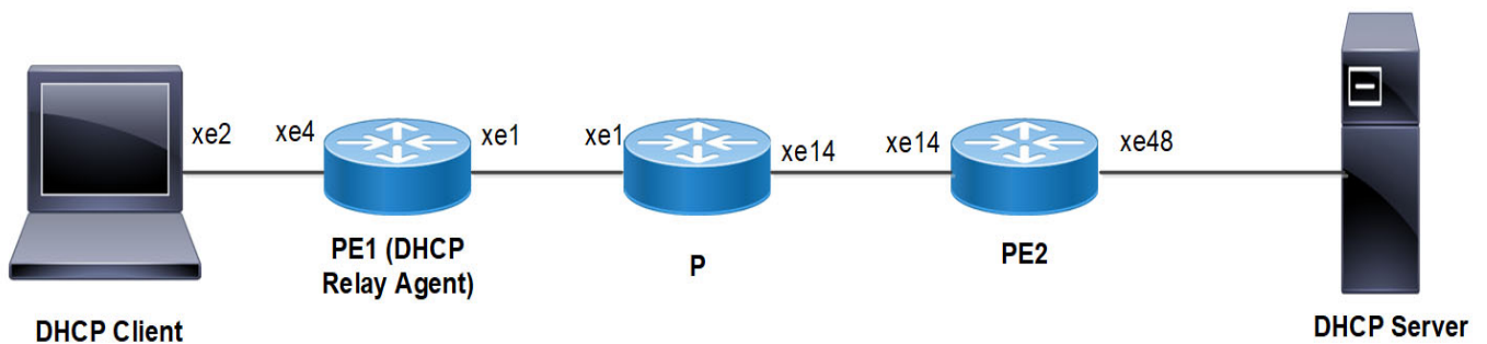
Figure 4-29: DHCP Relay Over L3 VPN Configuration
