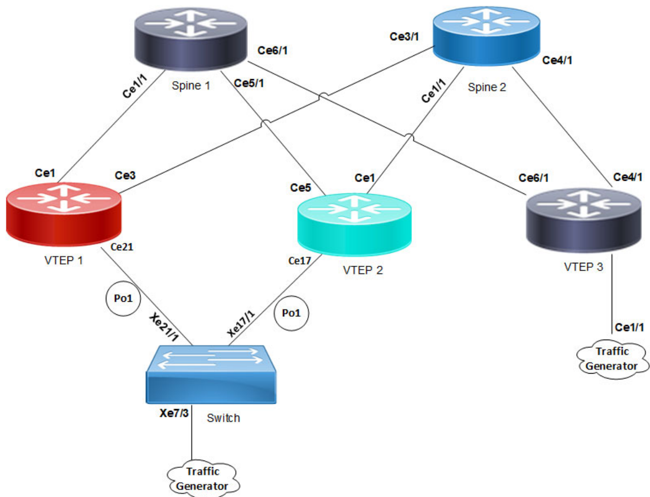
Figure 21-42: L2CP tunneling for VXLAN
