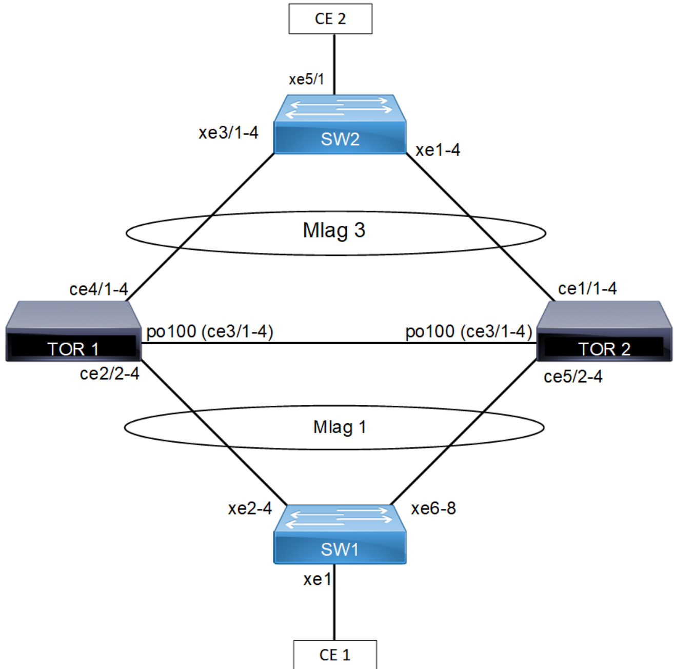
Figure 12-25: MLAG topology
