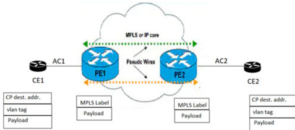
Figure 21-43: L2CP tunneling for VPLS/VPWS/Hybrid (bridge+VPWS)
