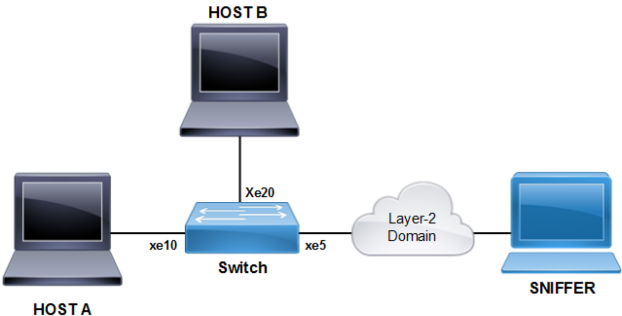
Figure 16-37: RSPAN Topology
