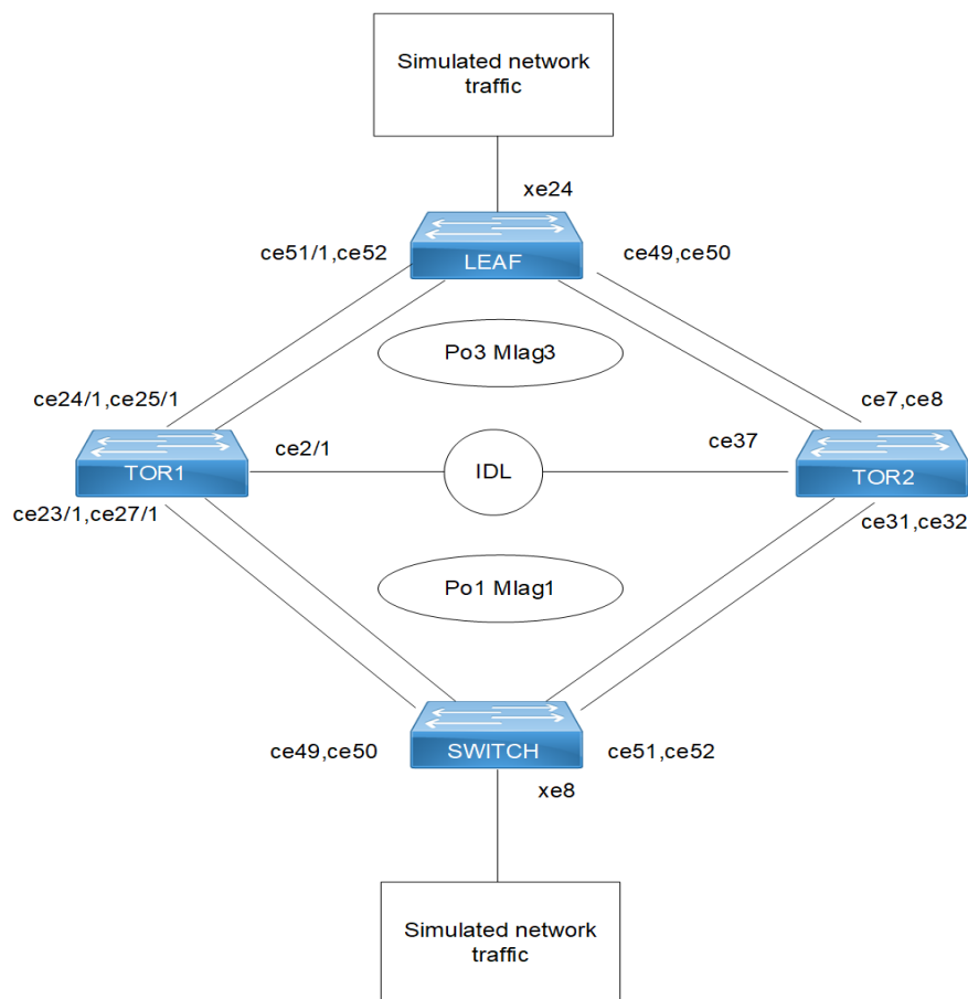
Figure 26-48: MLAG with Provider Bridging
