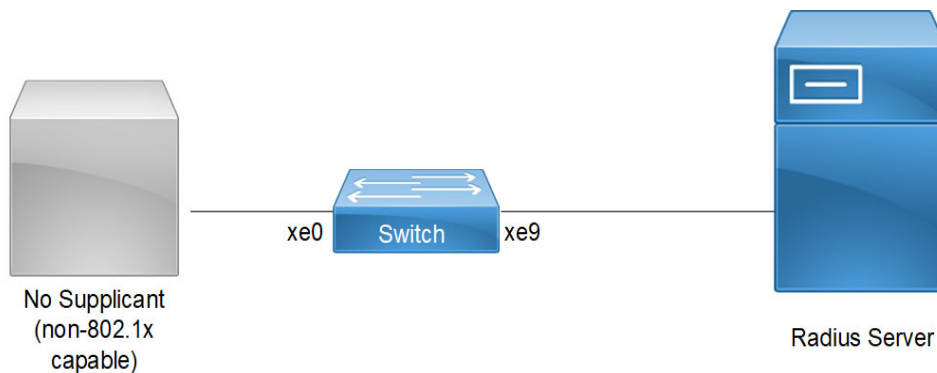
Figure 24-46: MAB Topology
