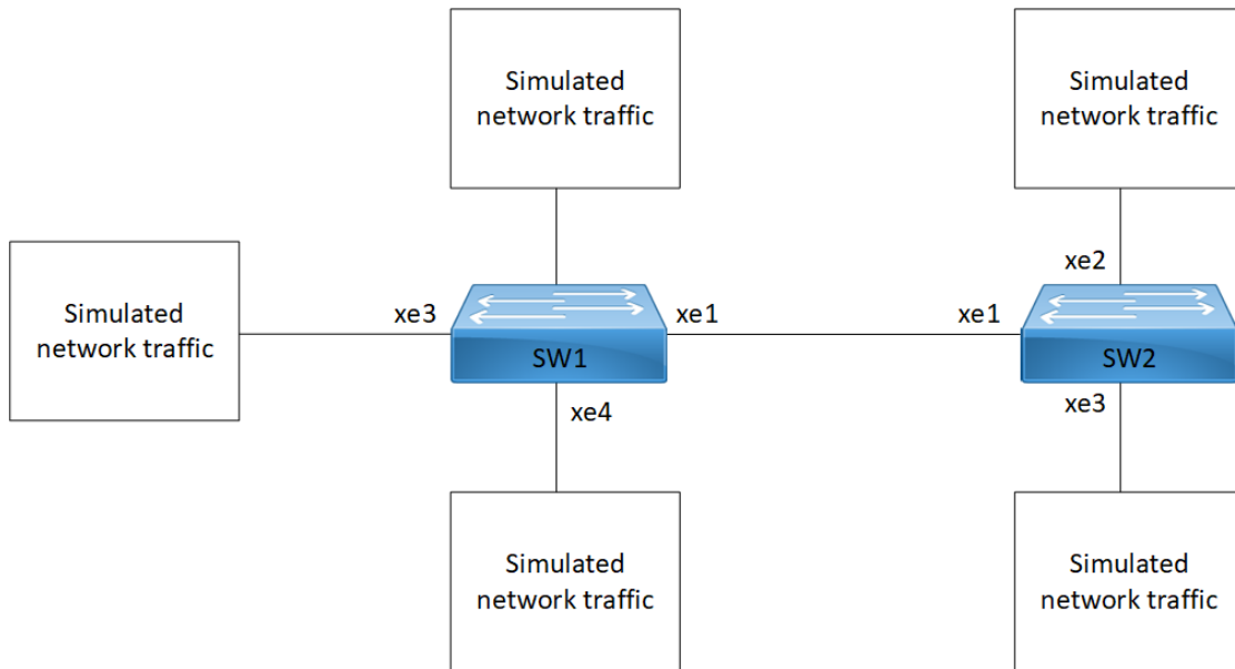
Figure 18-39: PVLAN configuration
