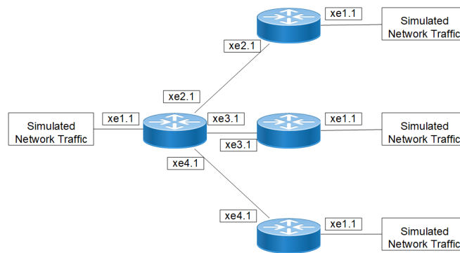
Figure 20-40: Bridging support over L2 subinterface
