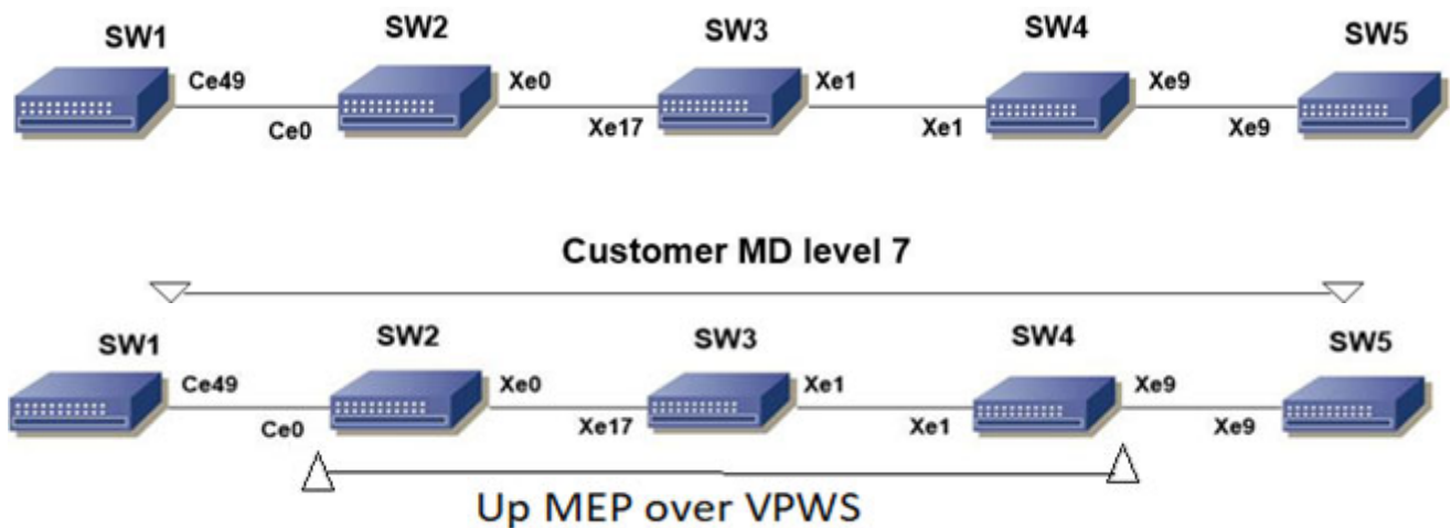
Figure 2-1: CFM Y.1731 Topology
