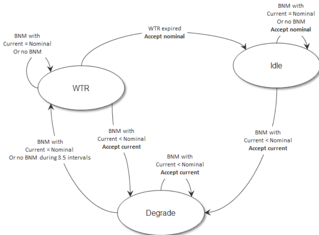
Figure 24-1: FSM Topology
