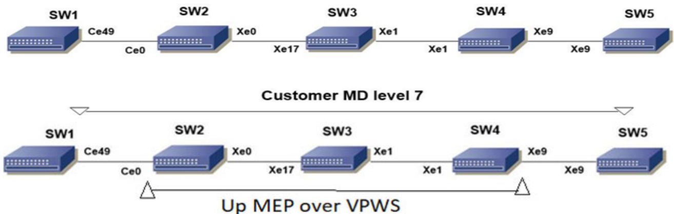
Figure 3-4: CFM Y.1731 LMM over L2 Bridge Topology
