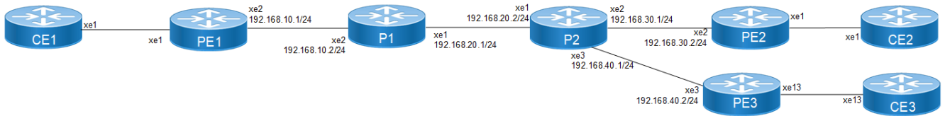
Figure 8-1: EVPN ELAN Over Sub-interface-Single Home
