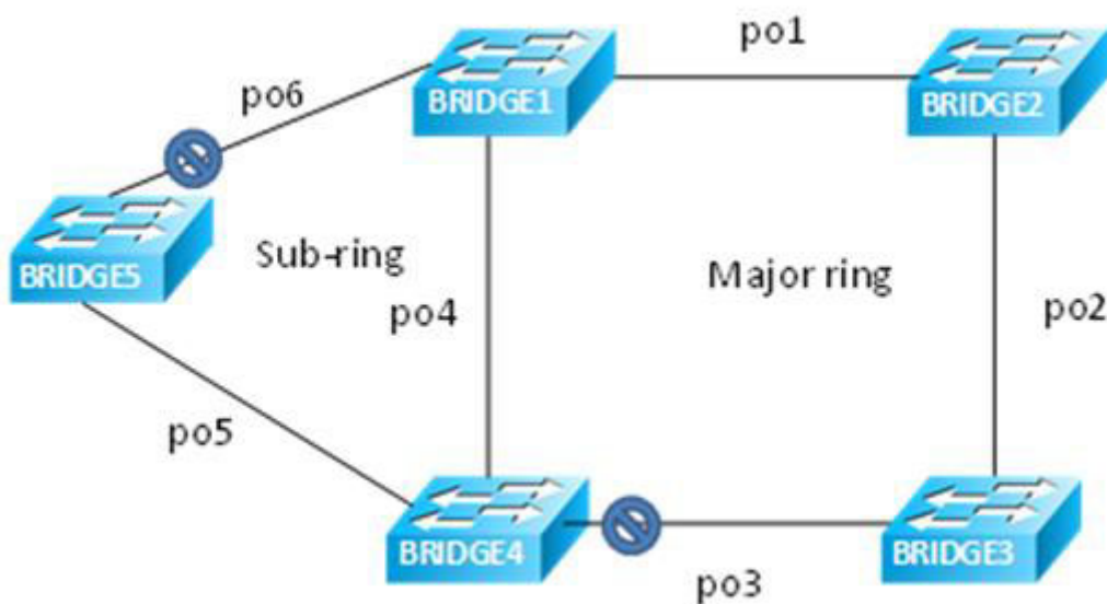
Figure 13-3: Major ring and sub-ring topology using LAG interface without a virtual channel
