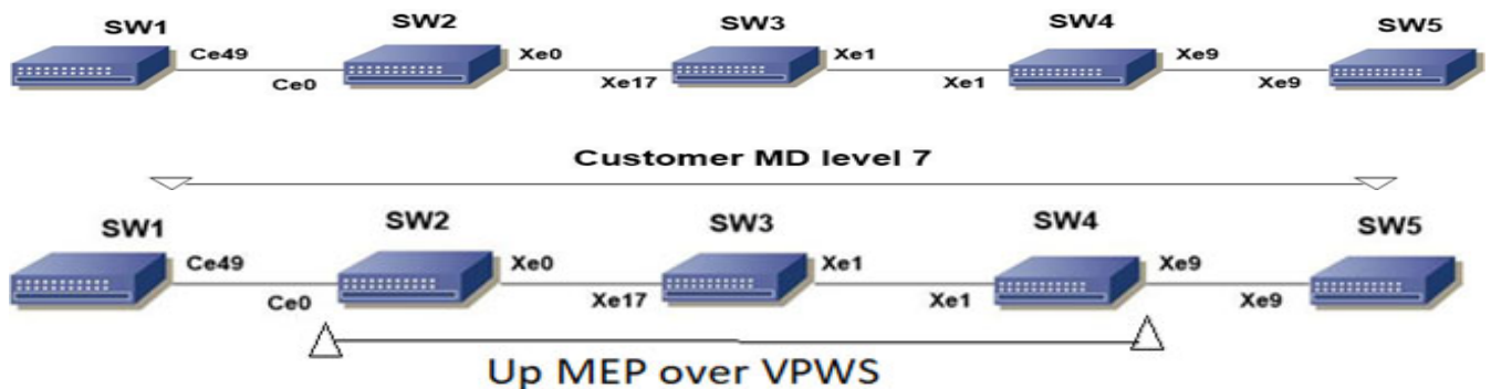
Figure 3-1: CFM Y.1731 SLM over L2 Bridge Topology
