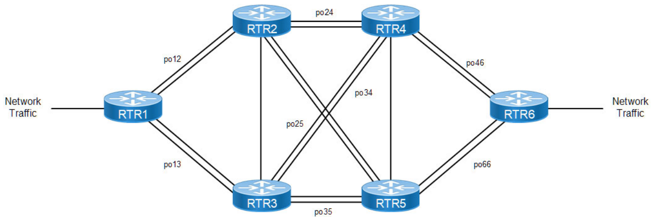
Figure 18-2: Simple Topology
