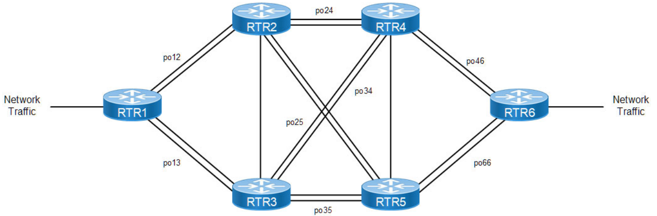
Figure 18-3: Simple Topology
