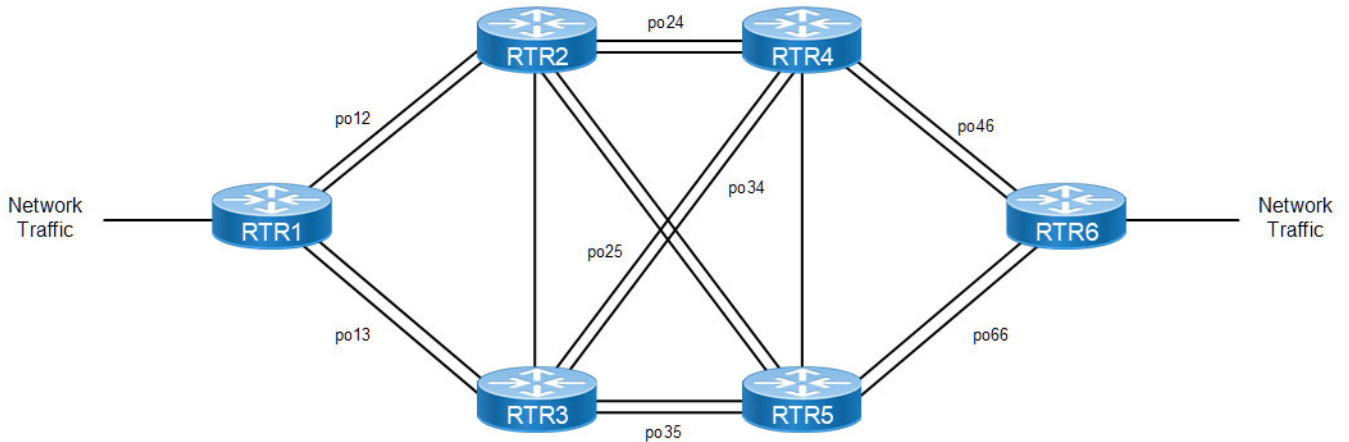
Figure 18-4: Simple Topology
