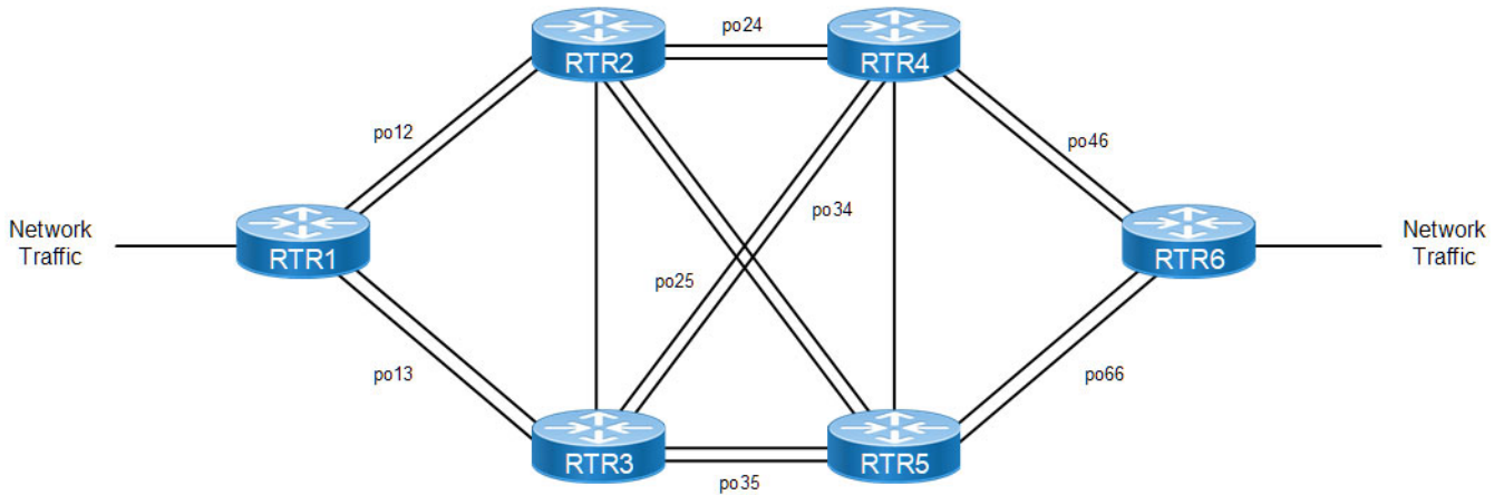
Figure 18-5: Simple Topology
