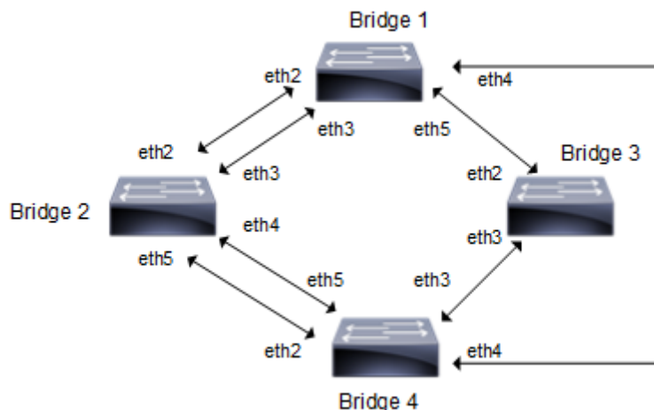
Figure 5-5: MSTP Topology
