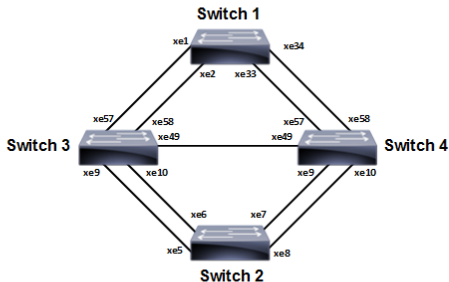
Figure 9-15: MLAG Topology
