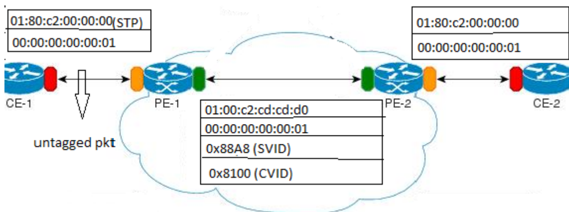
Figure 13-21: L2CP tunneling for provider bridging
