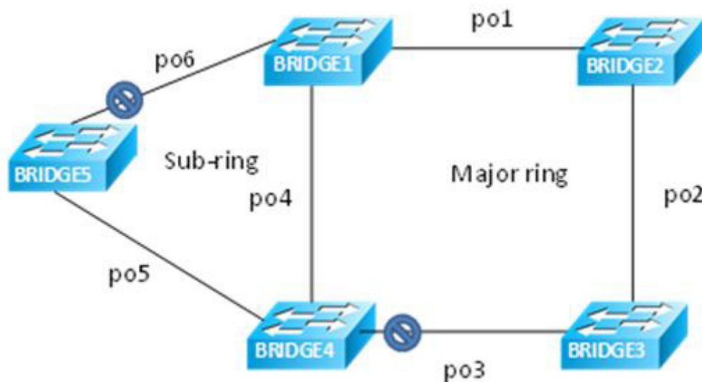
Figure 2-2: Major ring and sub-ring topology using LAG interface without a virtual channel
