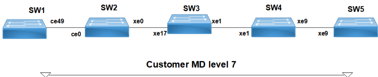
Figure 1-1: CFM Topology
