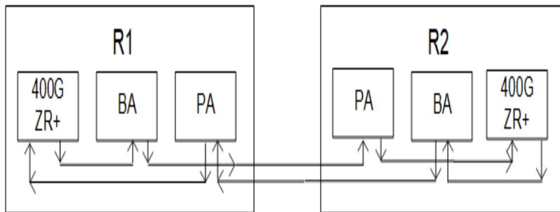
Figure 35-51: EDFA Sample Topology
