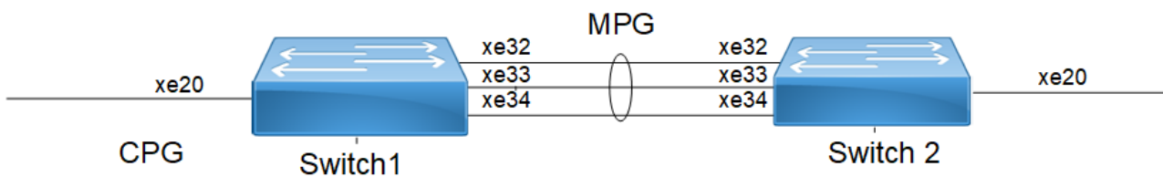
Figure 27-45: TFO with port-channel
