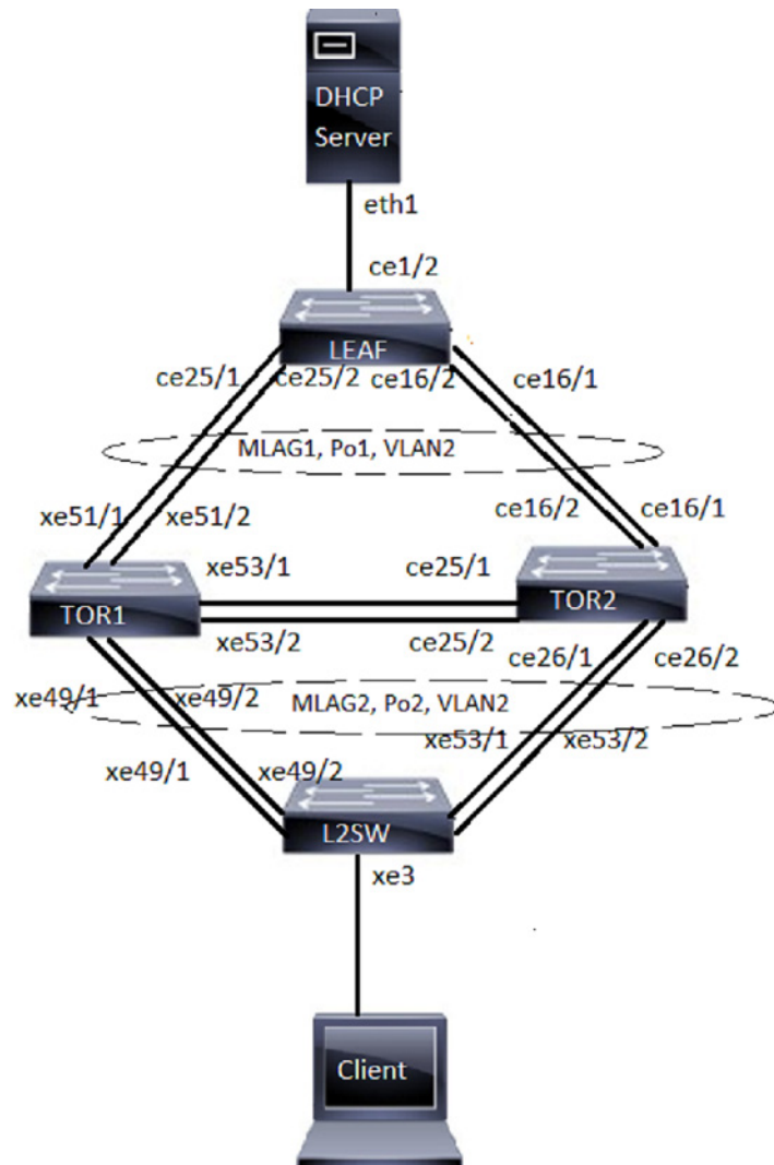
Figure 14-21: DHCP Snooping over MLAG
