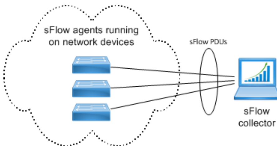
Figure 26-43: Basic sFlow topology
