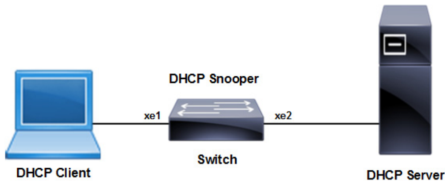
Figure 13-20: IP Source Guard Topology
