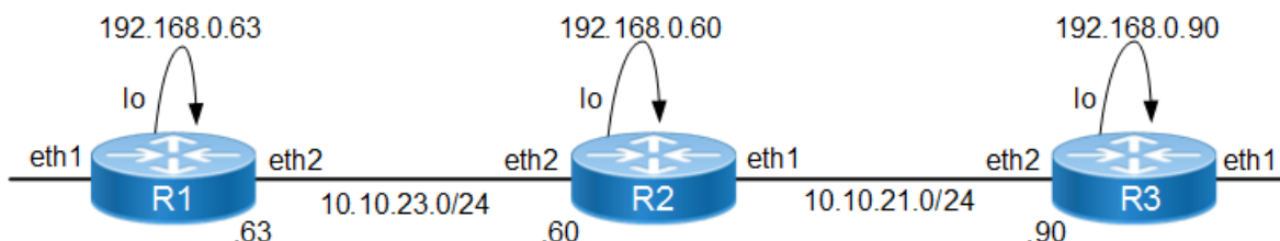
Figure 3-3: Basic Topology
