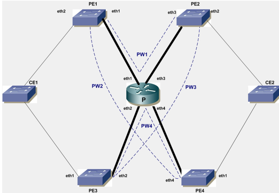
Figure 10-1: Dual-Homed CE Devices for Ethernet Pseudowires
