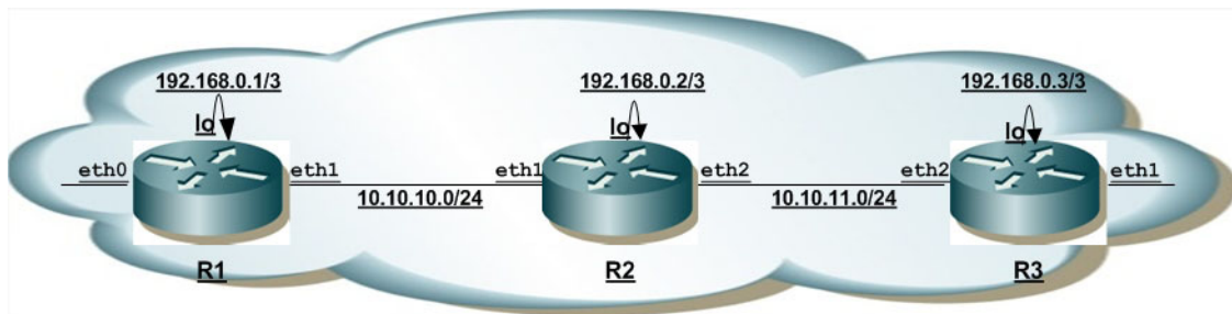
Figure 16-1: Basic Policing Topology
