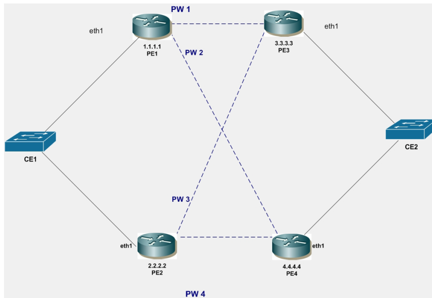
Figure 10-3: Multi-Homed CE with PW Redundancy for VLAN PW
