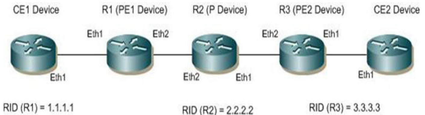
Figure 9-1: PW Topology
