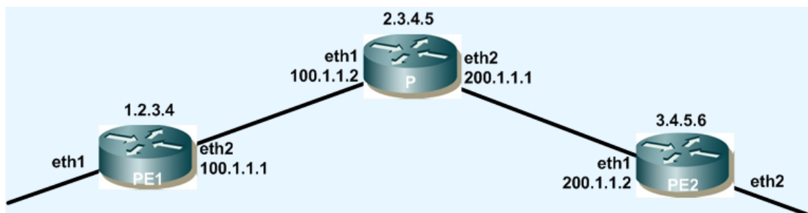
Figure 8-1: Topology for All Configurations
