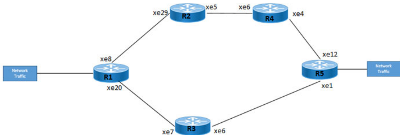
Figure 4-2: Facility Bypass with Ring Topology
