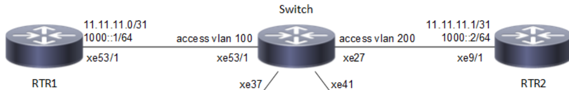
Figure 5-31: BFD user-defined VRF
