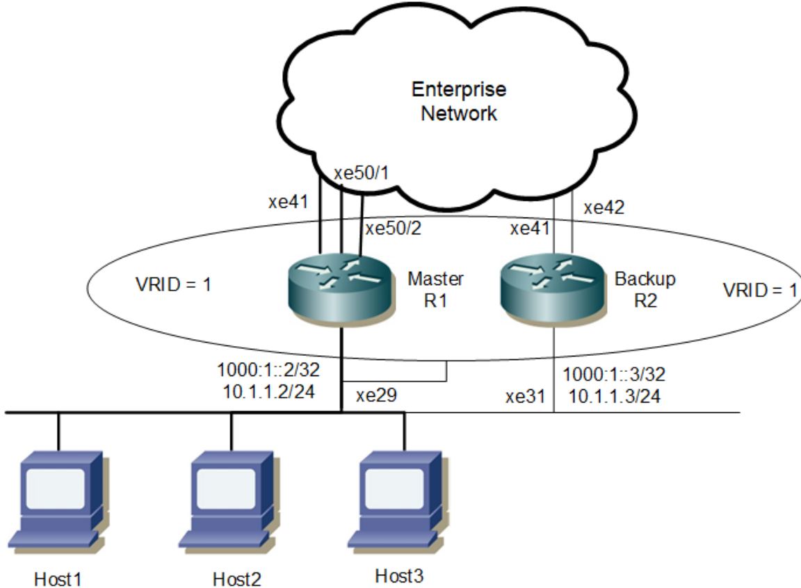
Figure 1-19: VRRP Interface Tracking
