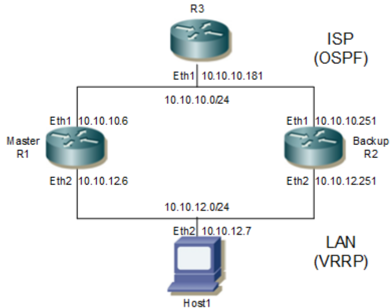
Figure 1-20: Redundancy Using VRRP and OSPF
