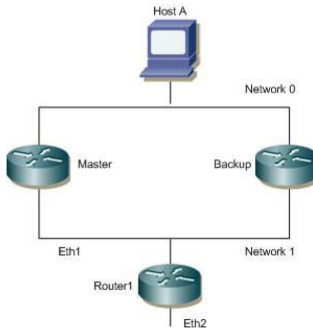
Figure 2-23: Topology
