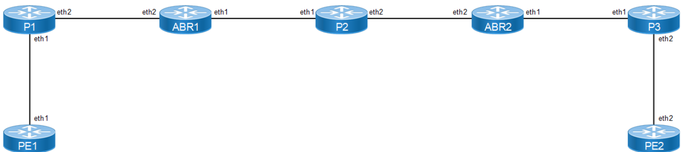
Figure 10-105: BGP_LU with MPLS
