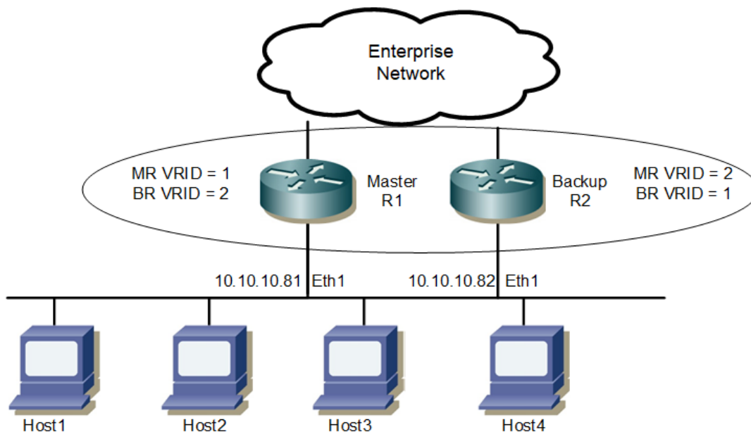
Figure 1-17: Configuring VRRP with Two Virtual Routers
