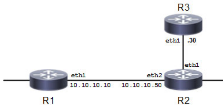
Figure 2-6: Multiple-key Topology
