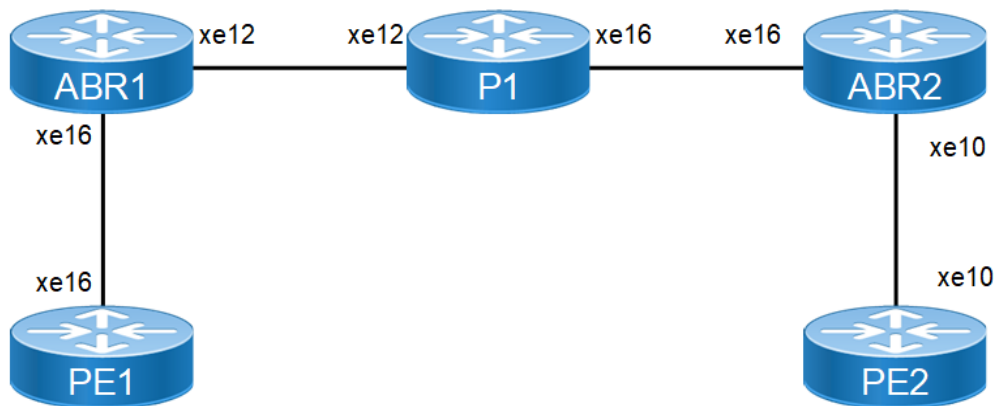
Figure 10-104: BGP labeled unicast
