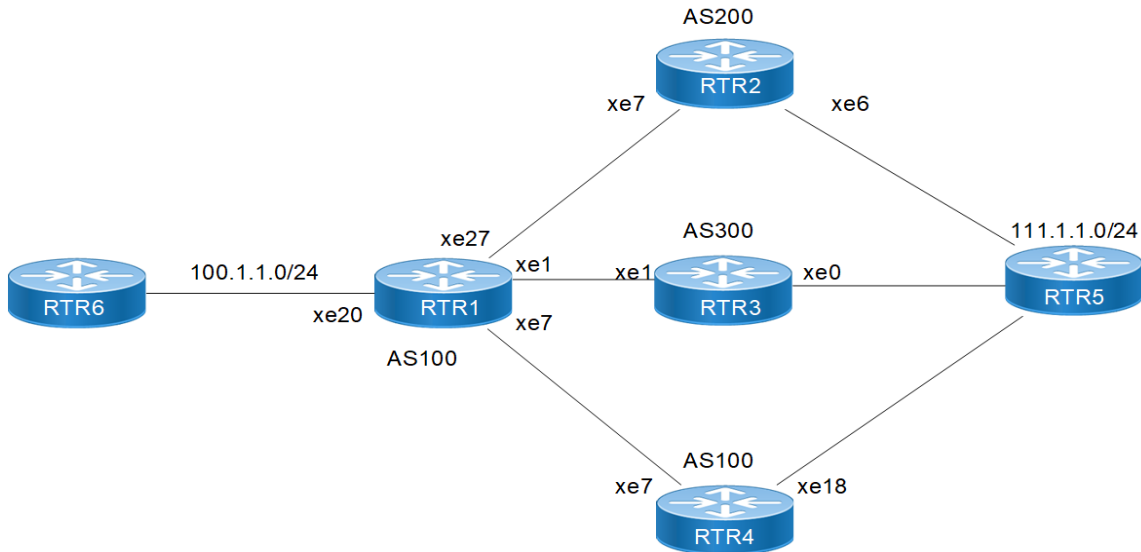
Figure 9-96: Multipath eBGP topology
