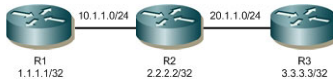
Figure 2-28: Basic Topology for BFD in BGP
