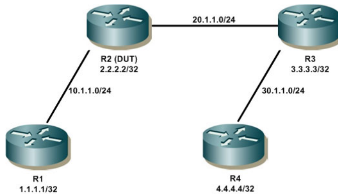
Figure 3-29: BFD Static Route Basic Topology
