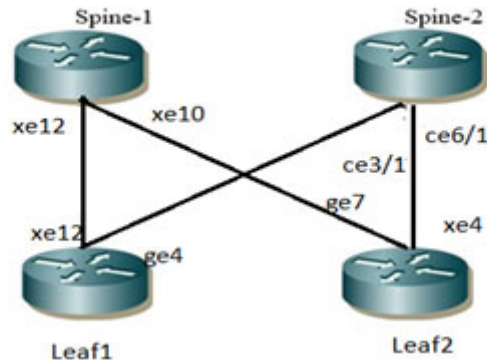
Figure 9-102: BGP-Unnumbered
