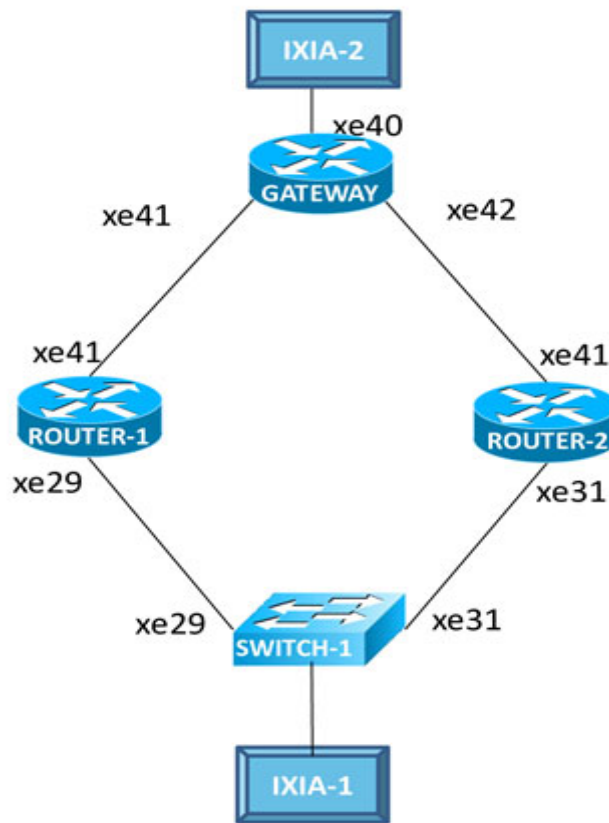
Figure 1-22: VRRP Object Tracking
