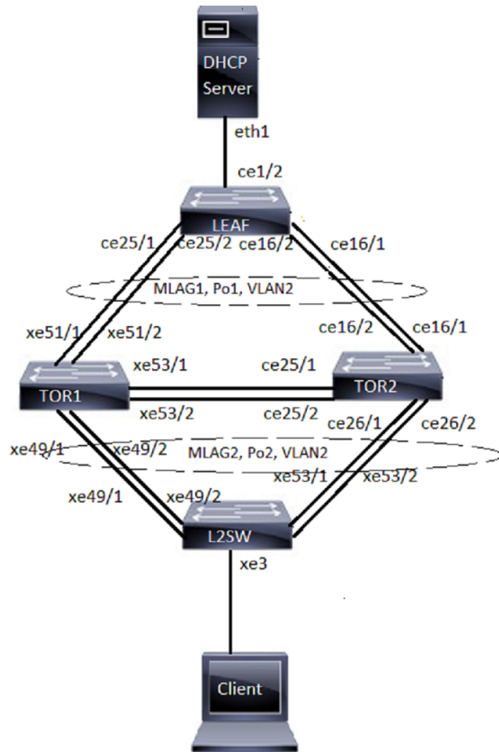
Figure 71. DHCP 1 Snooping over MLAG
