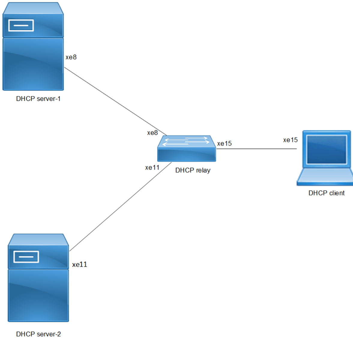
Figure 2-1: DHCP server group topology
