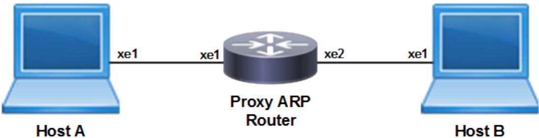
Figure 67. Sample topology
