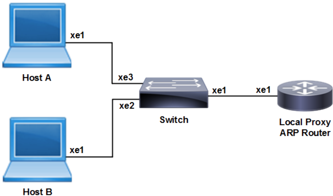
Figure 68. Sample topology
