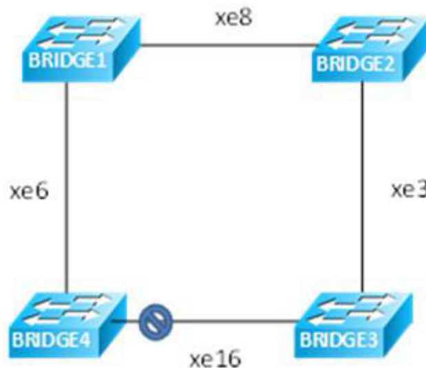
Figure 1-1: Major Ring Topology
