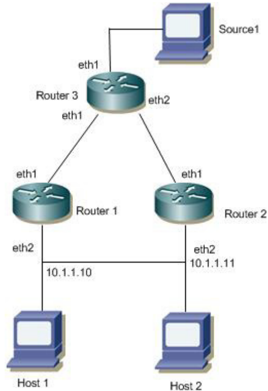
Figure 2-1: IGMP Topology
