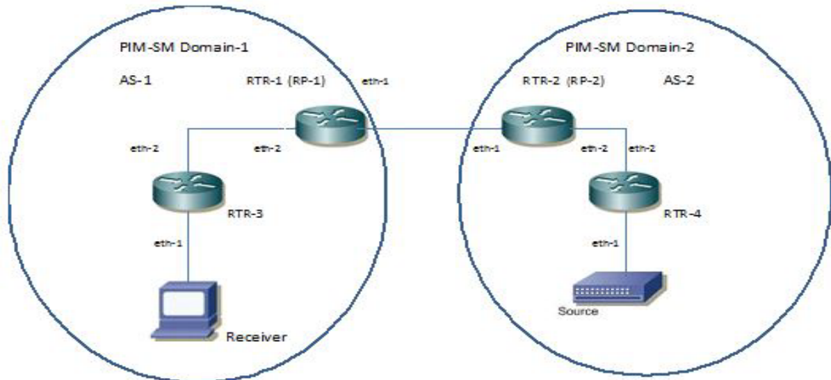
Figure 8-9: MSDP topology
