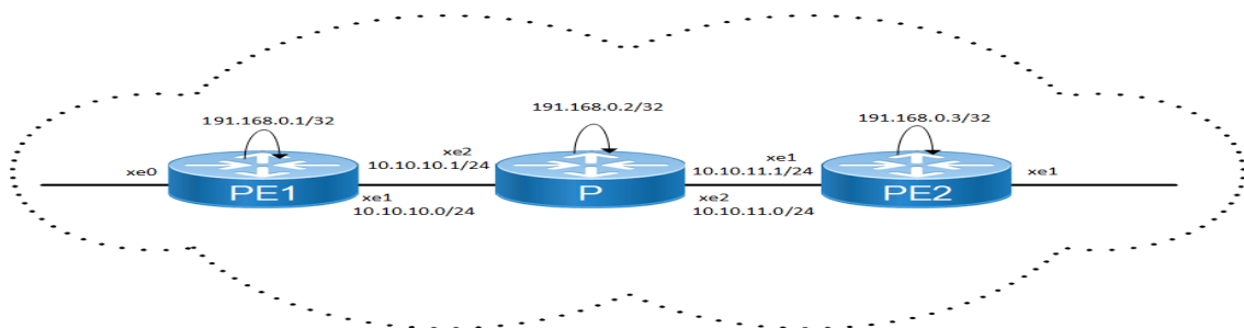
Figure 17-26: Basic Policing Topology
