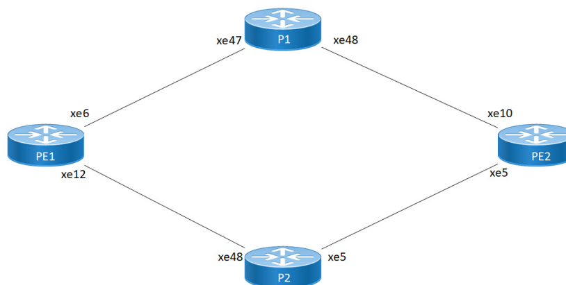
Figure 12-23: Basic LDP Topology
