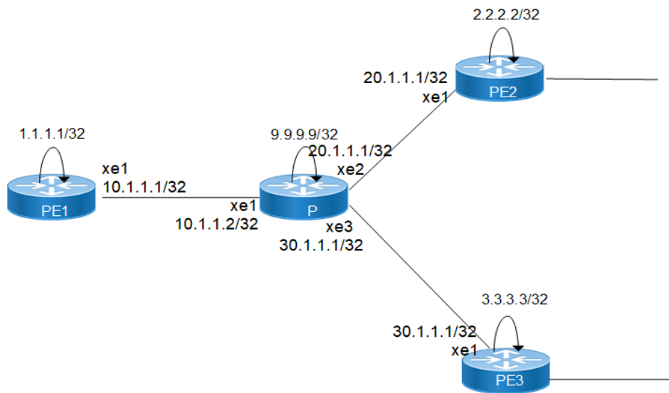
Figure 25-33: Static Virtual Private LAN Service Topology
