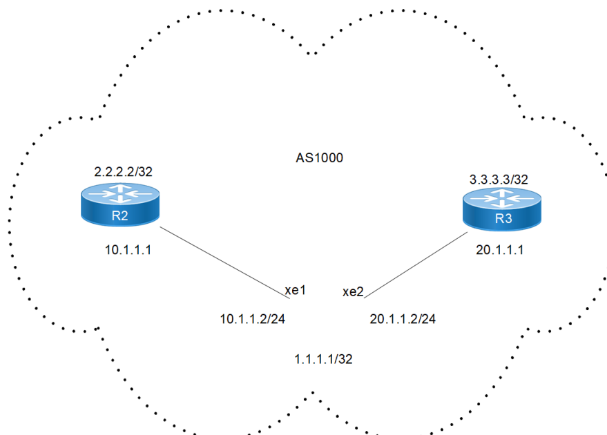
Figure 30-38: BGP Peer-Groups with L2VPN EVPN address-family
