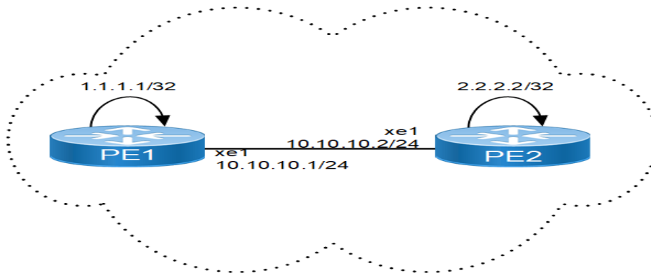
Figure 12-20: Topology for Direct Session MD5
