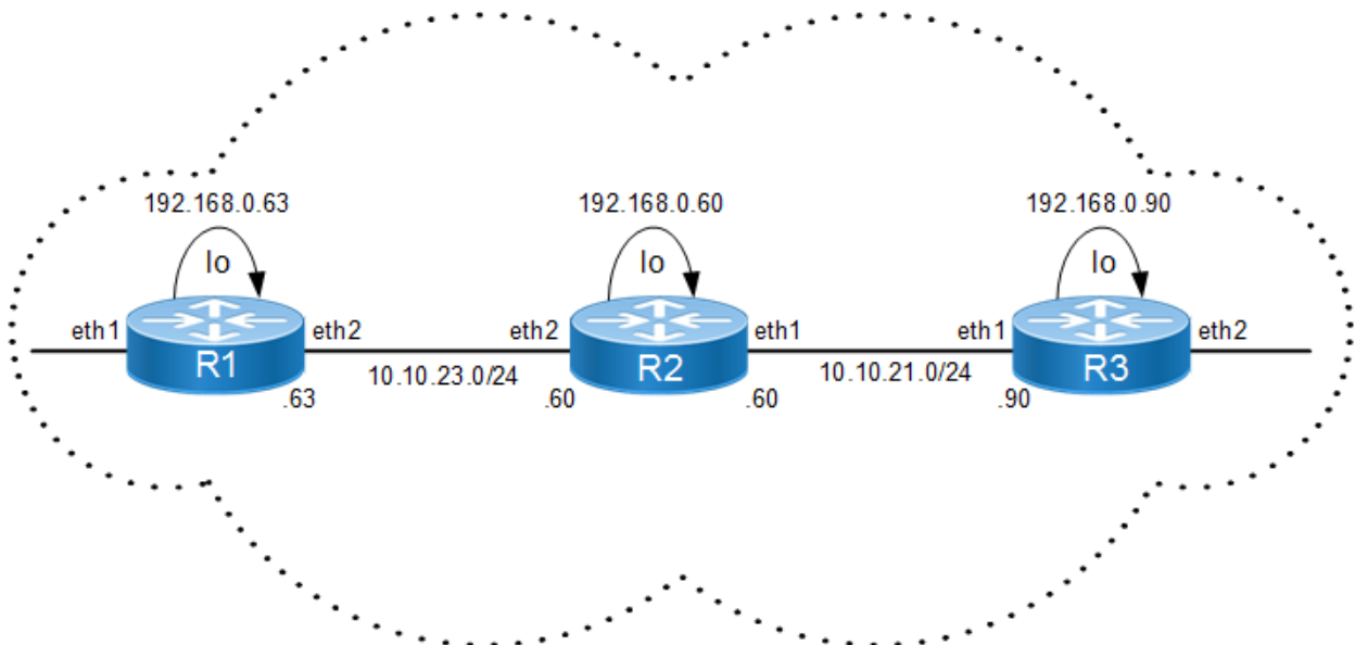
Figure 8-12: Topology for route mapping
