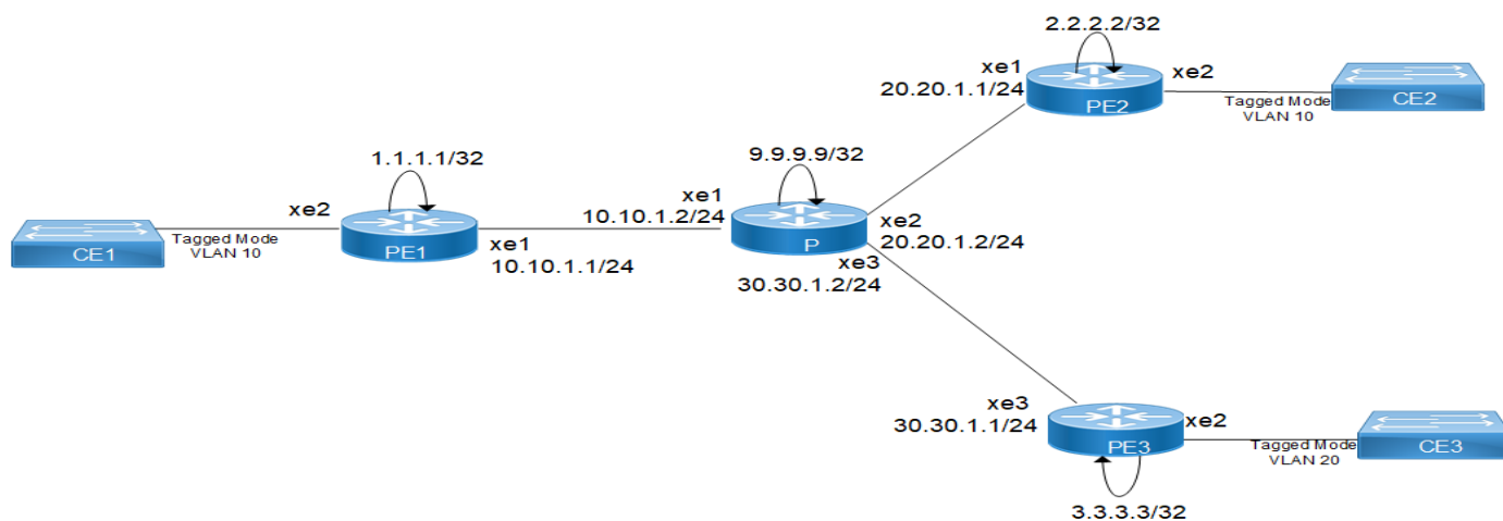
Figure 24-32: VPLS Mesh Peers Tagged Mode
