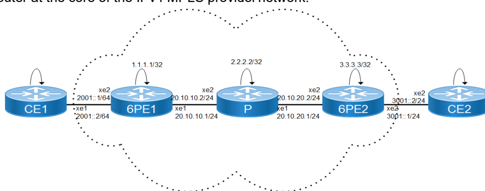
Figure 7-8: 6VPE Configuration
