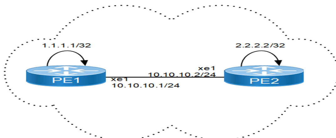
Figure 12-22: LDP Session Topology
