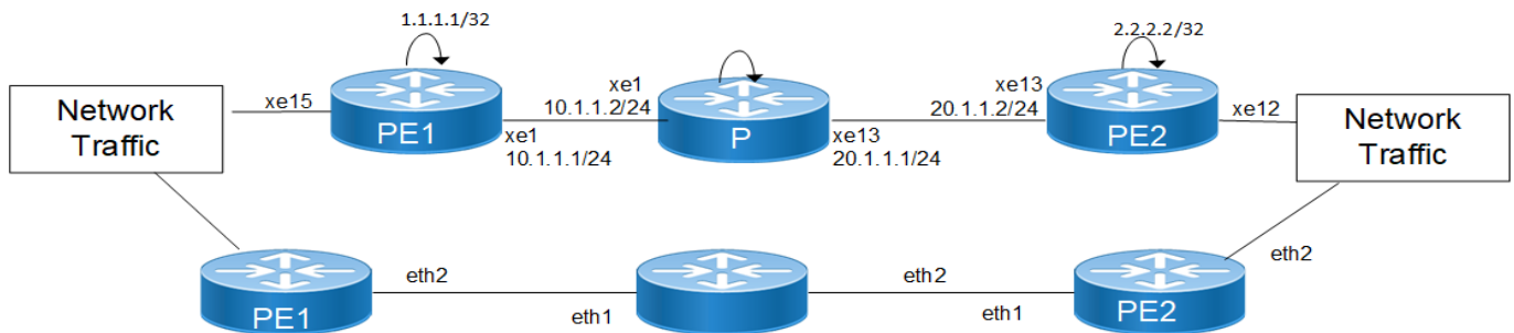
Figure 22-29: Mapping of RSVP Tunnel-name to L2VPN services
