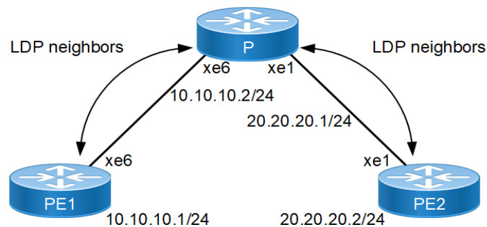
Figure 1-1: LDP Topology
