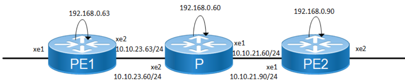
Figure 8-11: Basic Topology
