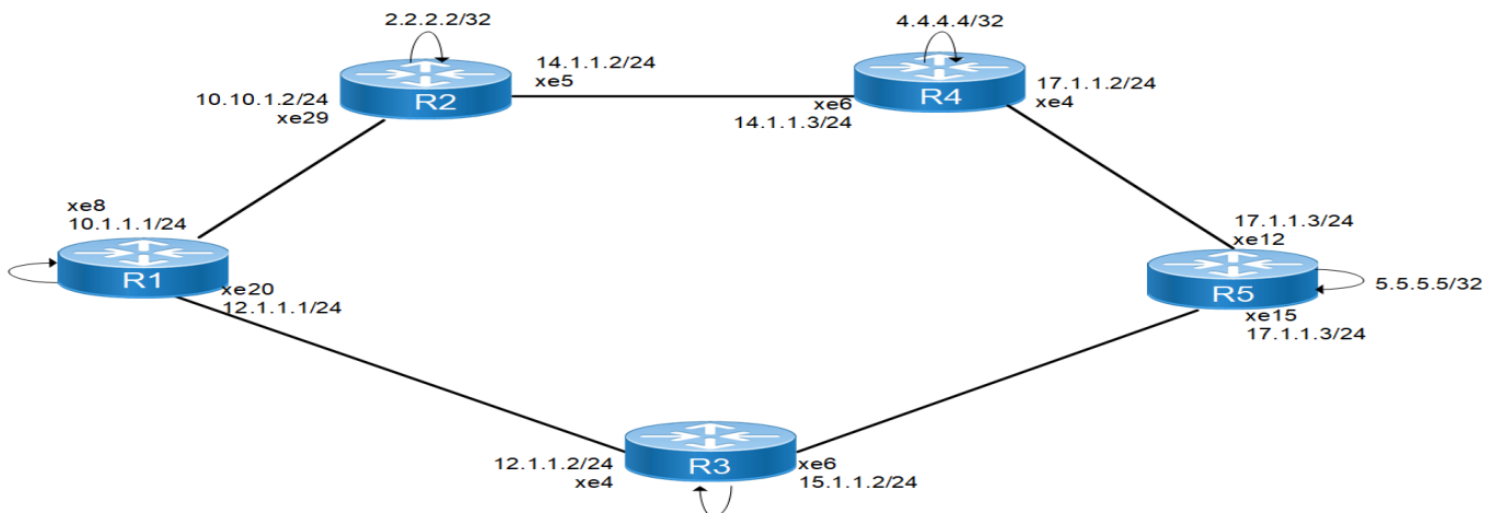
Figure 11-18: Facility Bypass with Ring Topology
