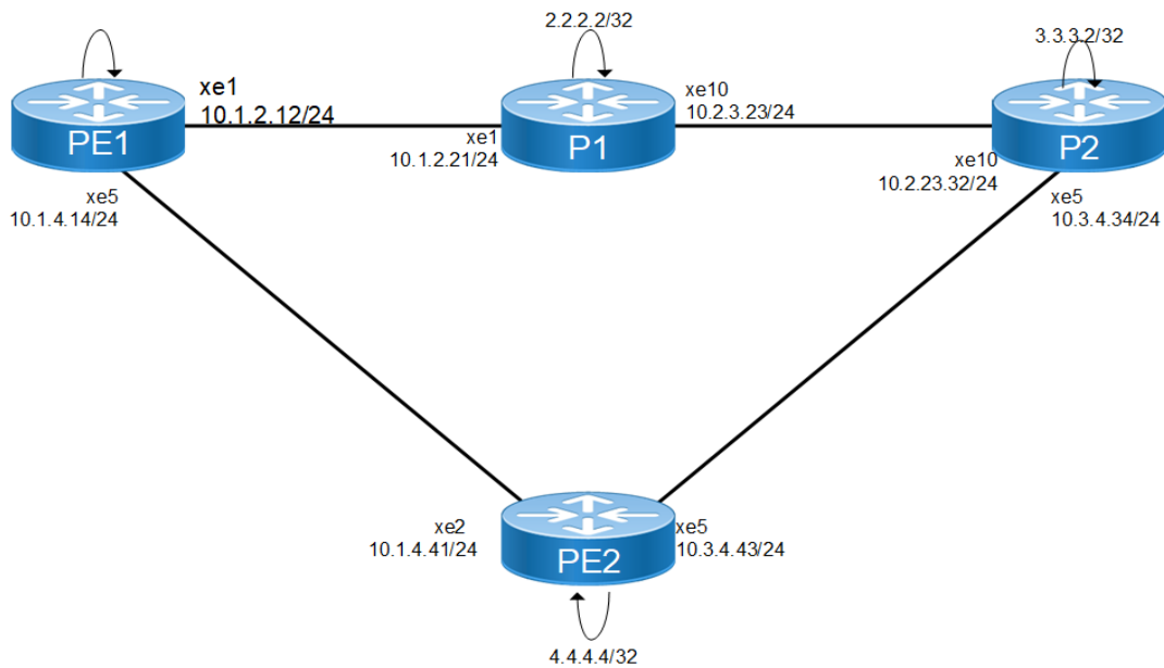
Figure 11-17: RSVP facility backup
