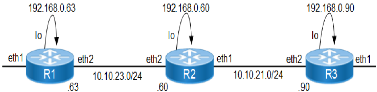
Figure 23-30: Minimal configuration Topology
