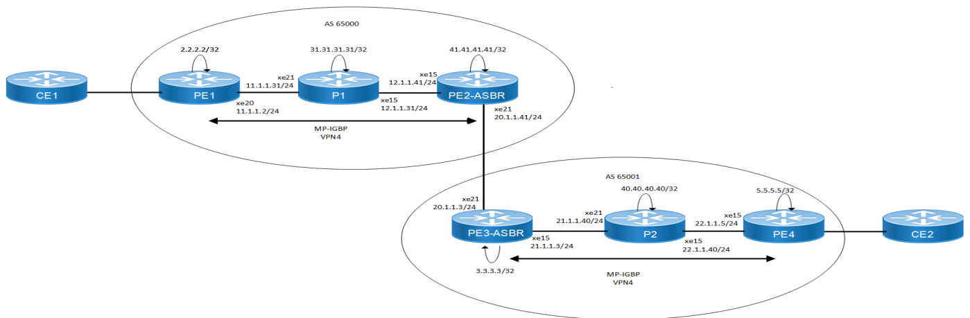
Figure 20-28: InterAS-VPN Option-A
