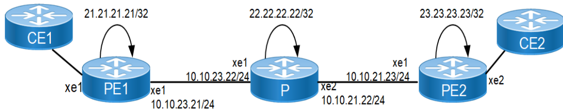
Figure 28-36: LDP-VPLS SM
