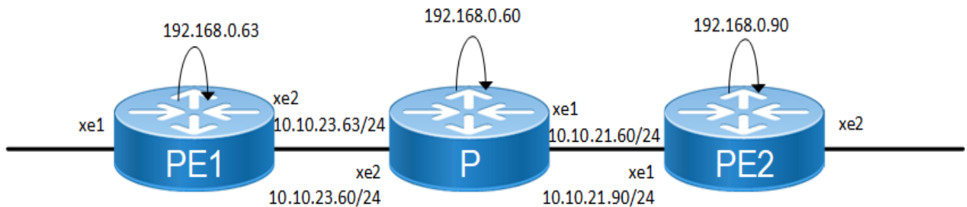
Figure 8-10: Topology for Minimal Configuration
