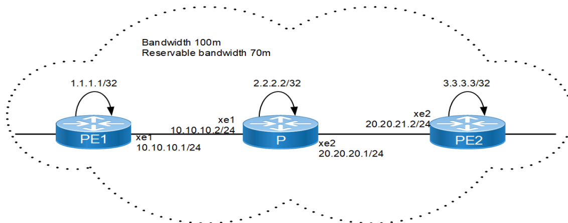
Figure 12-21: Topology for Targeted Session MD5
