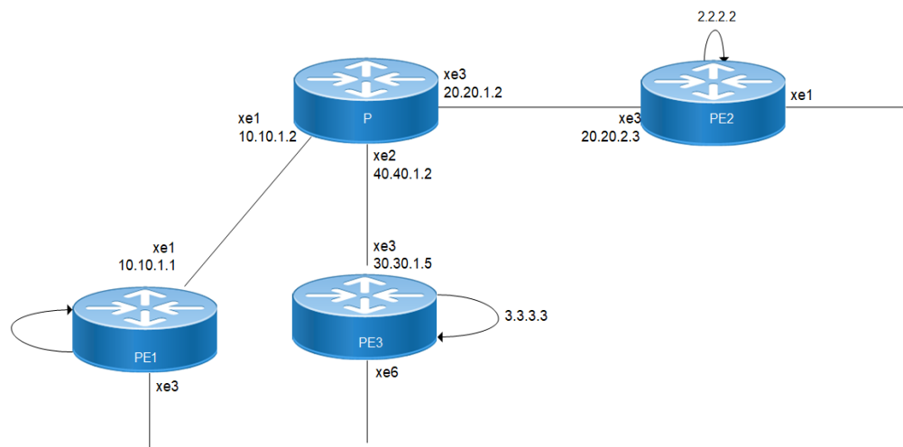
Figure 26-34: Sample Topology for VPLS with BGP Signaling
