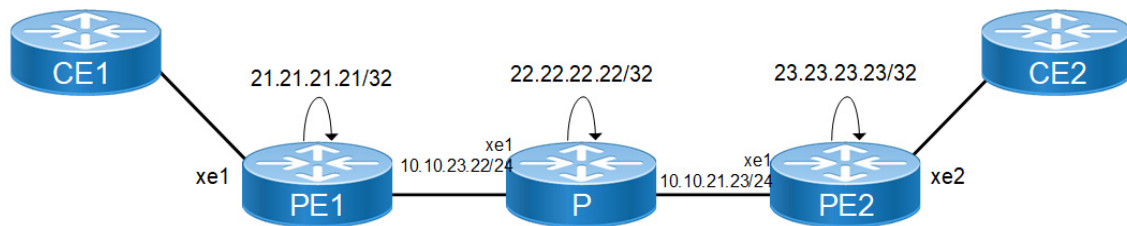
Figure 27-35: Static VPLS Service Mapping
