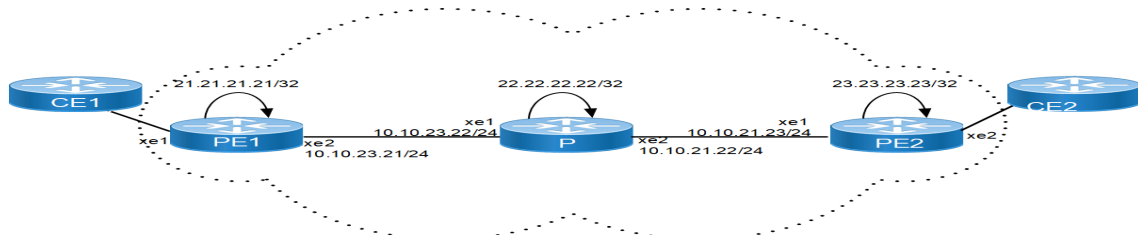
Figure 29-37: BGP-VPLS SM
