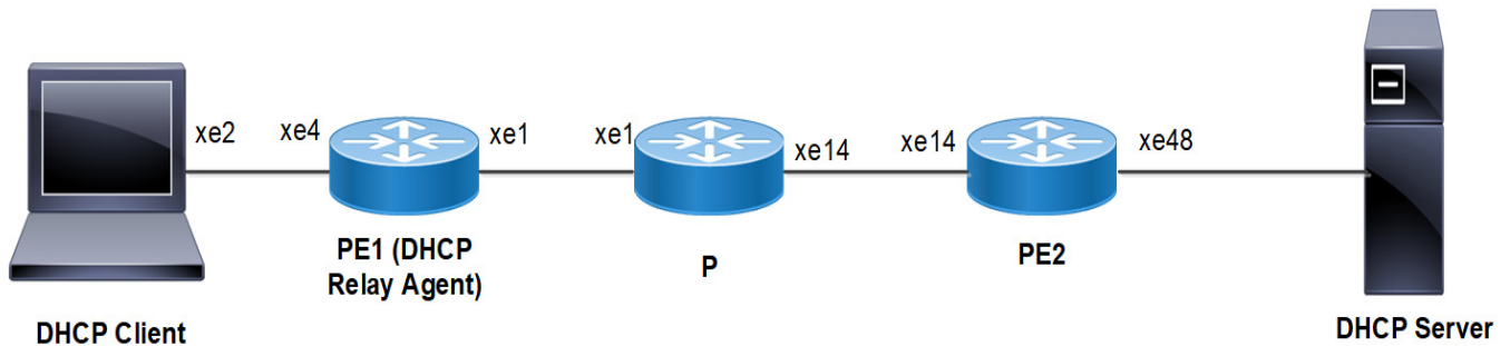
Figure 31-39: DHCP Relay Over L3 VPN Configuration
