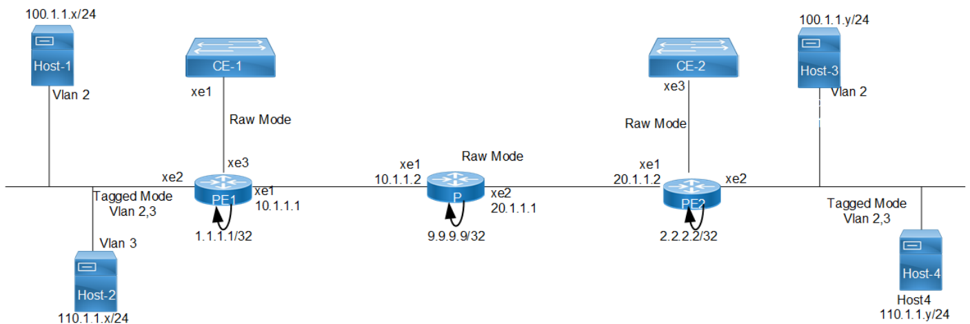
Figure 3-3: MPLS Layer 2 Virtual Circuit
