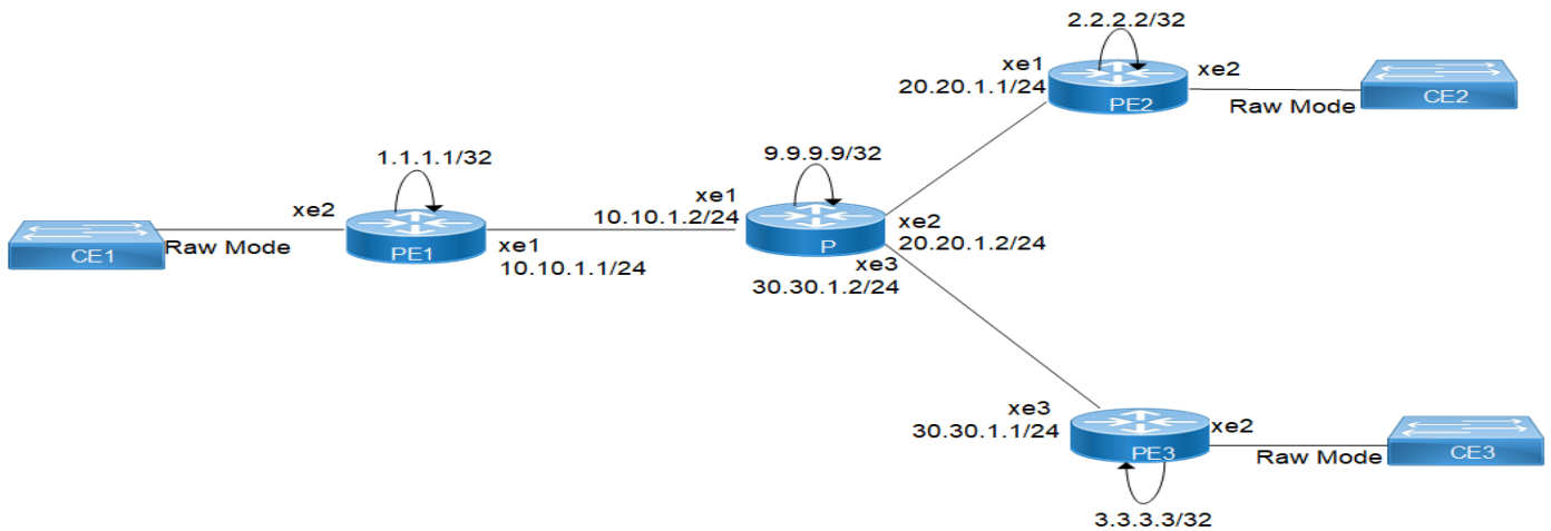
Figure 24-31: VPLS Mesh Peers Raw Mode
