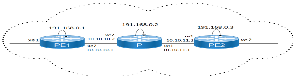
Figure 16-25: Basic LDP Topology
