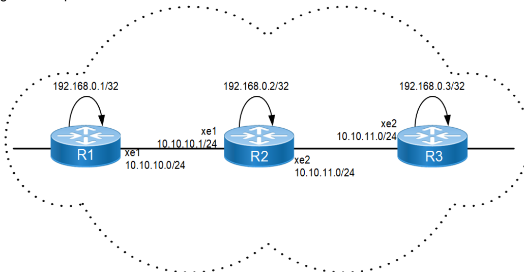
Figure 12-19: Basic LDP Topology
