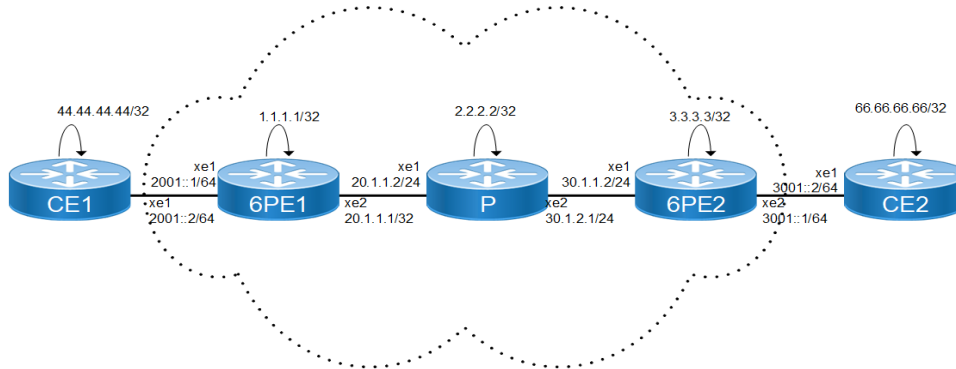
Figure 6-7: 6PE Configuration
