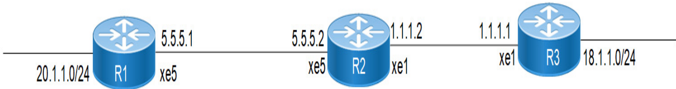
Figure 10-105: BGP Blackhole Community Attribute topology
