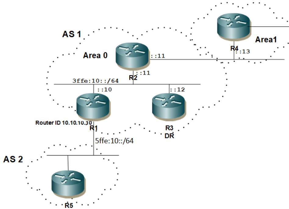
Figure 5-28: OSPFv3 Redistribute Routes
