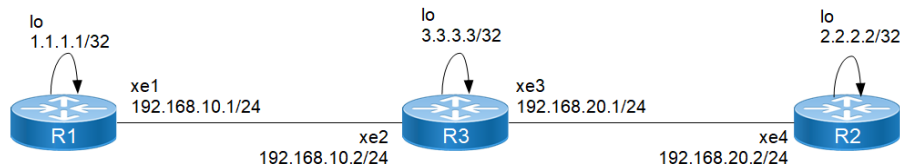
Figure 7-52: Configure Overload Bit Suppress
