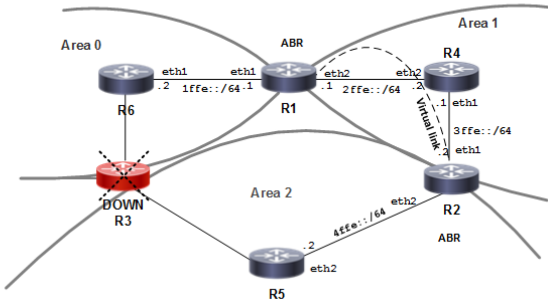
Figure 5-30: OSPFv3 Virtual Links
