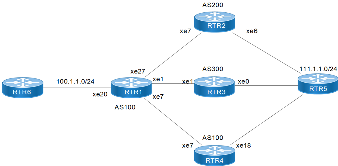
Figure 10-98: Multipath eBGP topology
