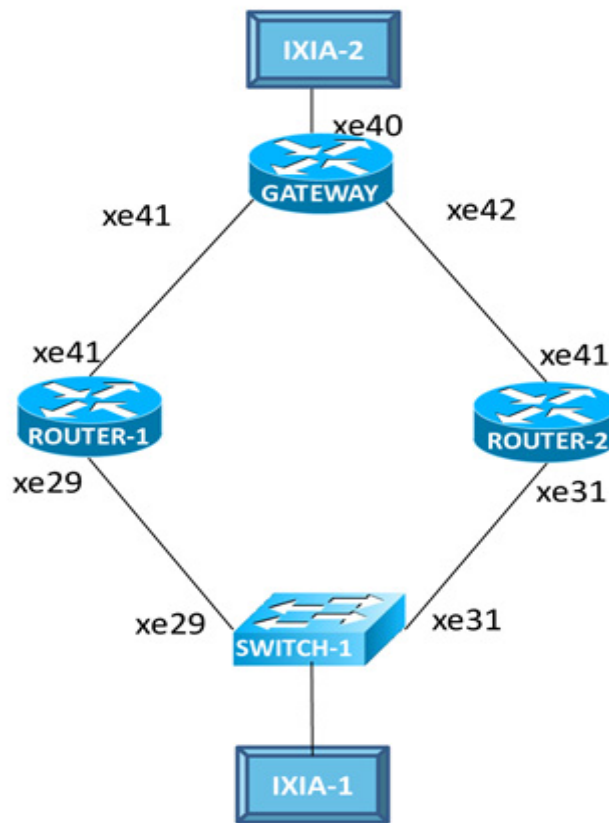
Figure 1-17: VRRP Object Tracking
