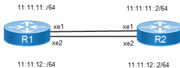
Figure 10-77: IPv6 IBGP Peering
