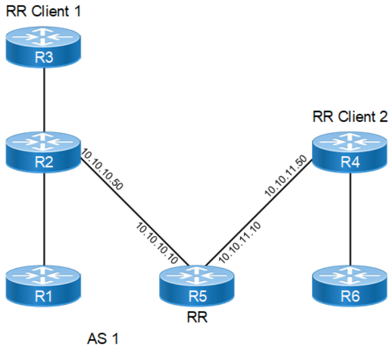
Figure 10-69: BGP Route Reflector
