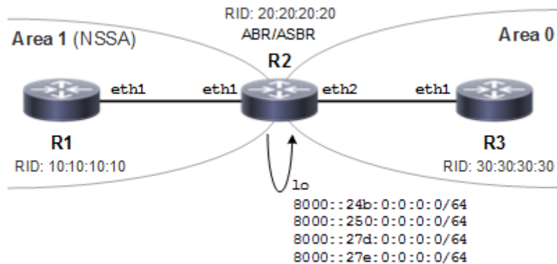
Figure 5-32: NSSA with Route Options
