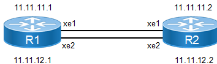
Figure 10-74: IPv4 IBGP Peering
