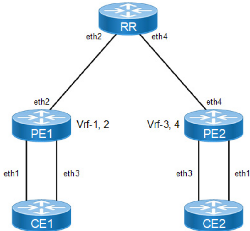
Figure 10-101: Route-target Filter Topology
