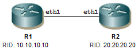
Figure 5-35: LSA Suppression
