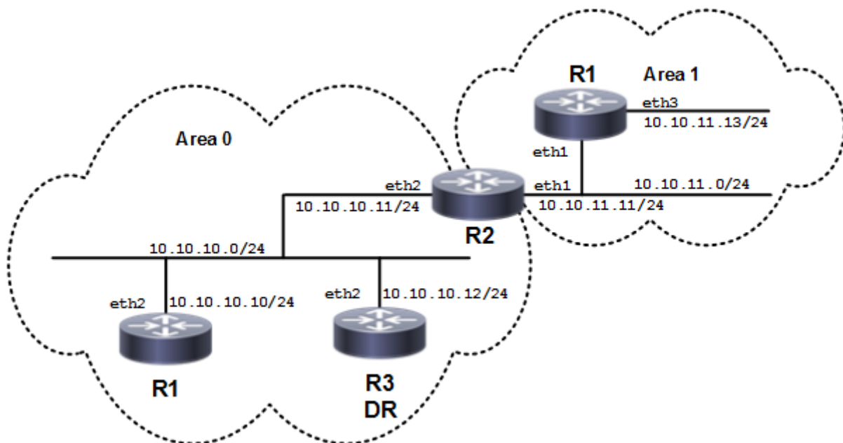
Figure 4-10: OSPF ABR Topology
