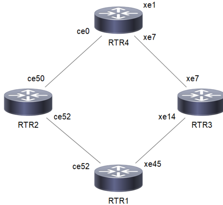
Figure 14-2: Static Route Object Tracking
