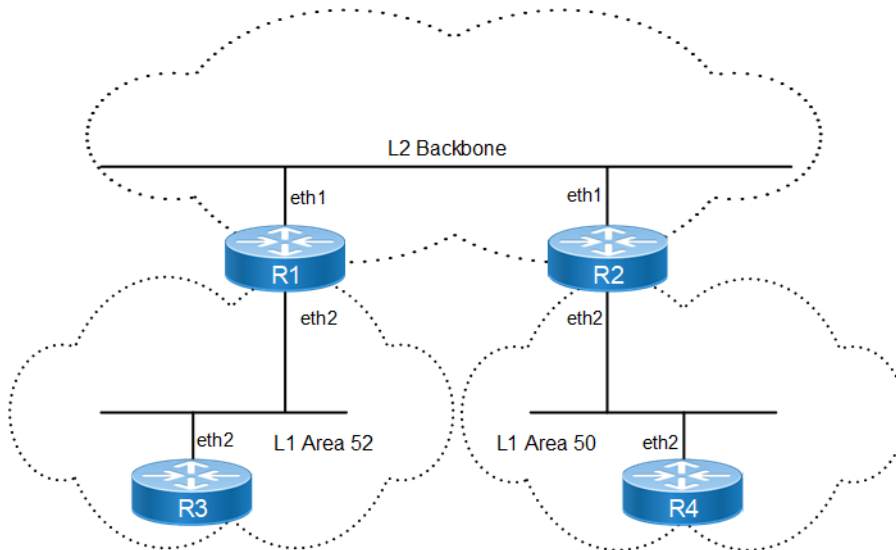
Figure 7-46: Single-Instance L1-L2 Area Routing
