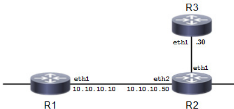
Figure 2-6: MD5 Multiple-key Topology
