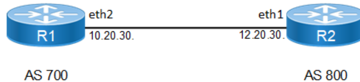
Figure 10-88: 4-Octet ASN
