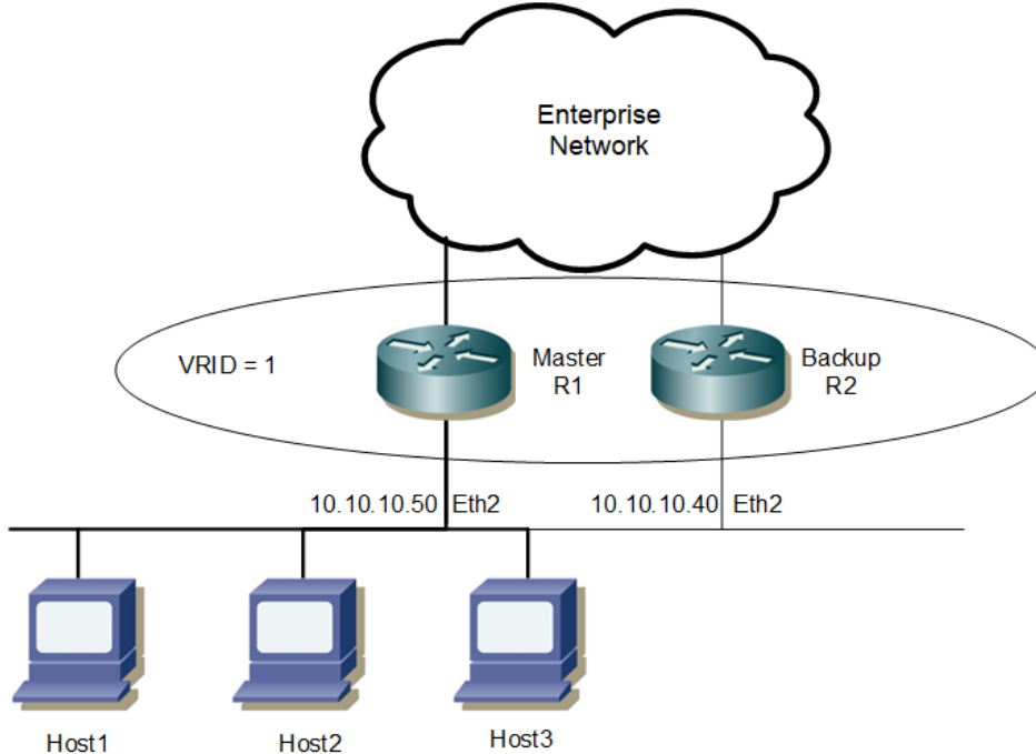
Figure 1-11: VRRP with One Virtual Router
