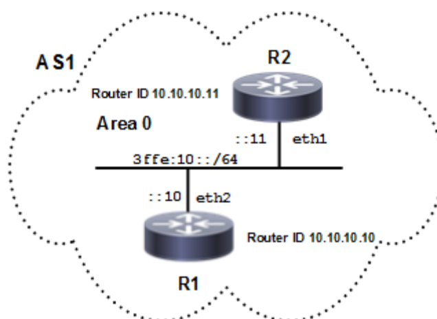
Figure 5-25: Basic OSPFv3 Topology
