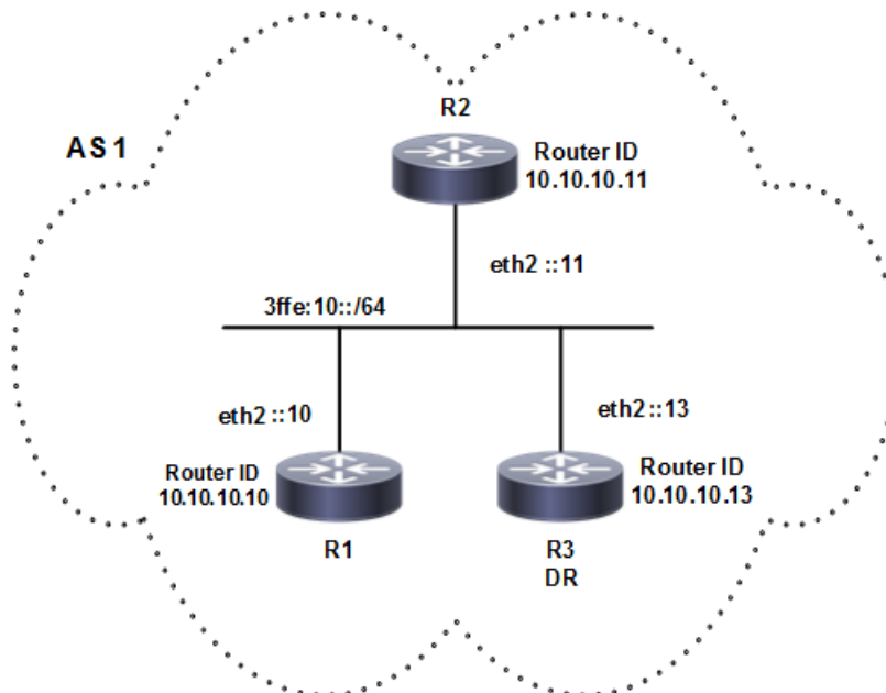
Figure 5-26: OSPFv3 Set Priority
