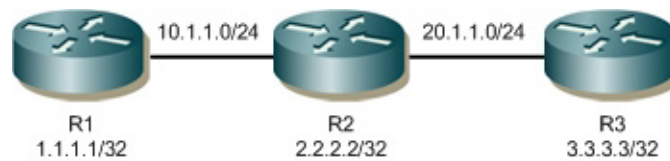
Figure P-22: Basic Topology for BFD in BGP
