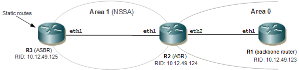
Figure 5-36: Originate Type-7 LSAs and Translate to Type-5 under Address Family IPv4
