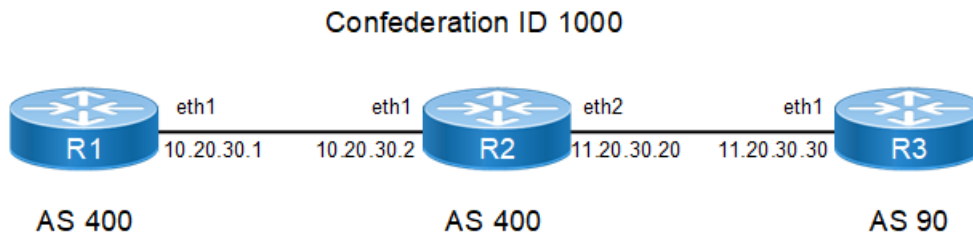
Figure 10-73: Single Confederation with Outside AS
