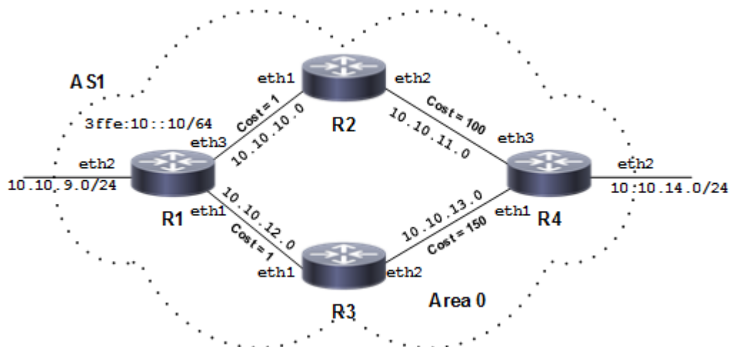
Figure 4-12: Configure Cost Topology
