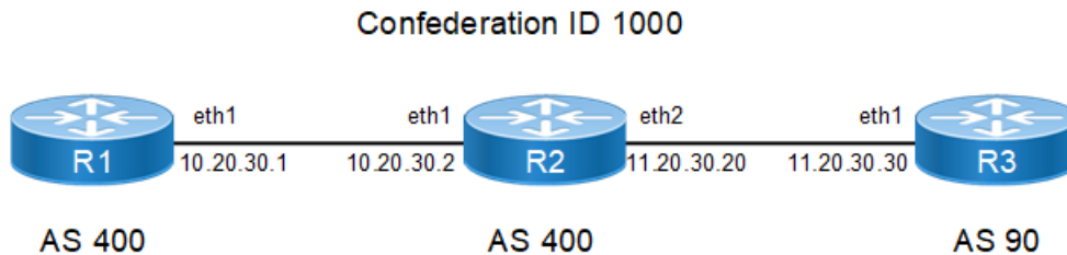
Figure 10-72: BGP Confederation with Multiple AS
