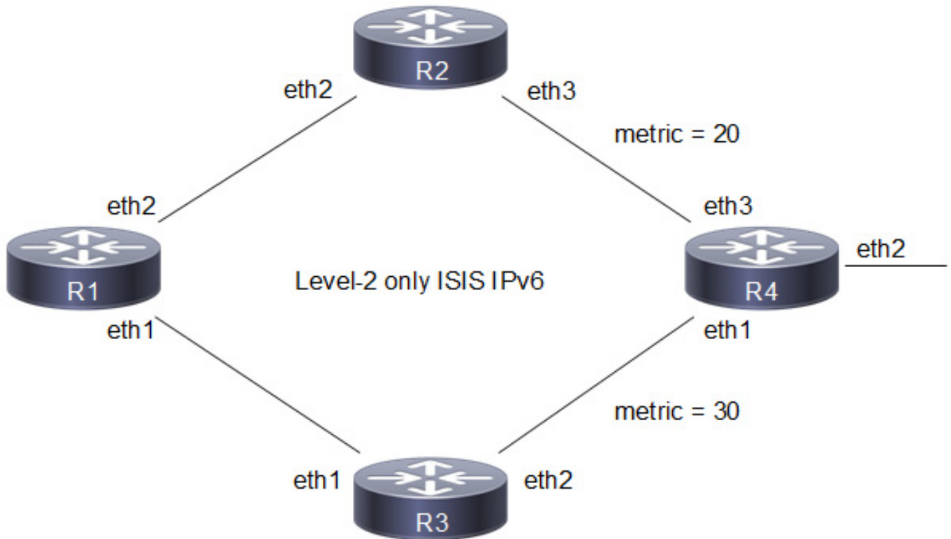
Figure 8-60: Configure IS-IS Metric
