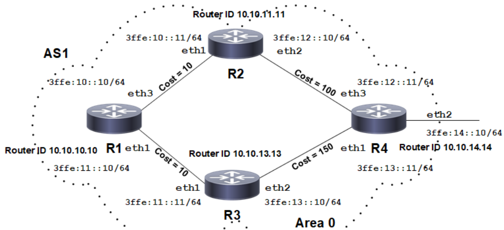
Figure 5-29: Configure Cost OSPFv3
