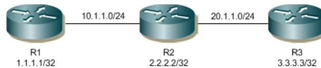
Figure P-19: Single-Hop OSPF Topology
