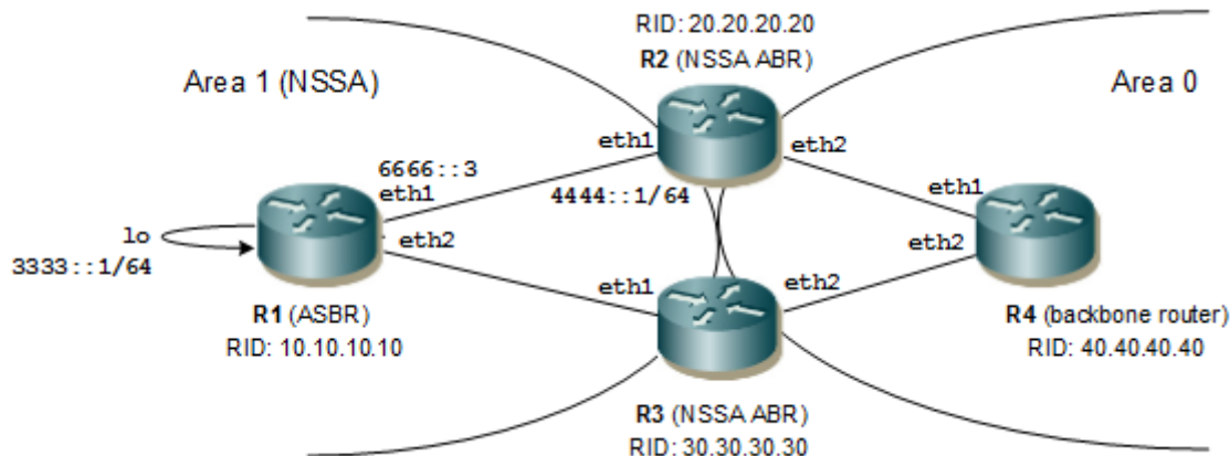
Figure 5-34: Using the translator-role Option
