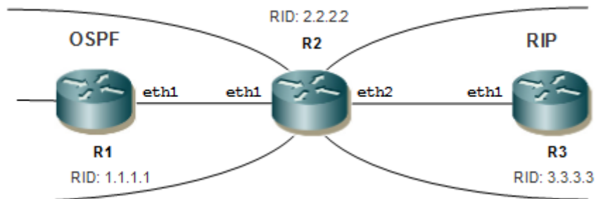
Figure 5-38: Basic Topology for Distribute-list
