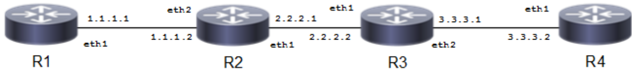
Figure 4-18: One Subnet with Multiple OSPF Areas
