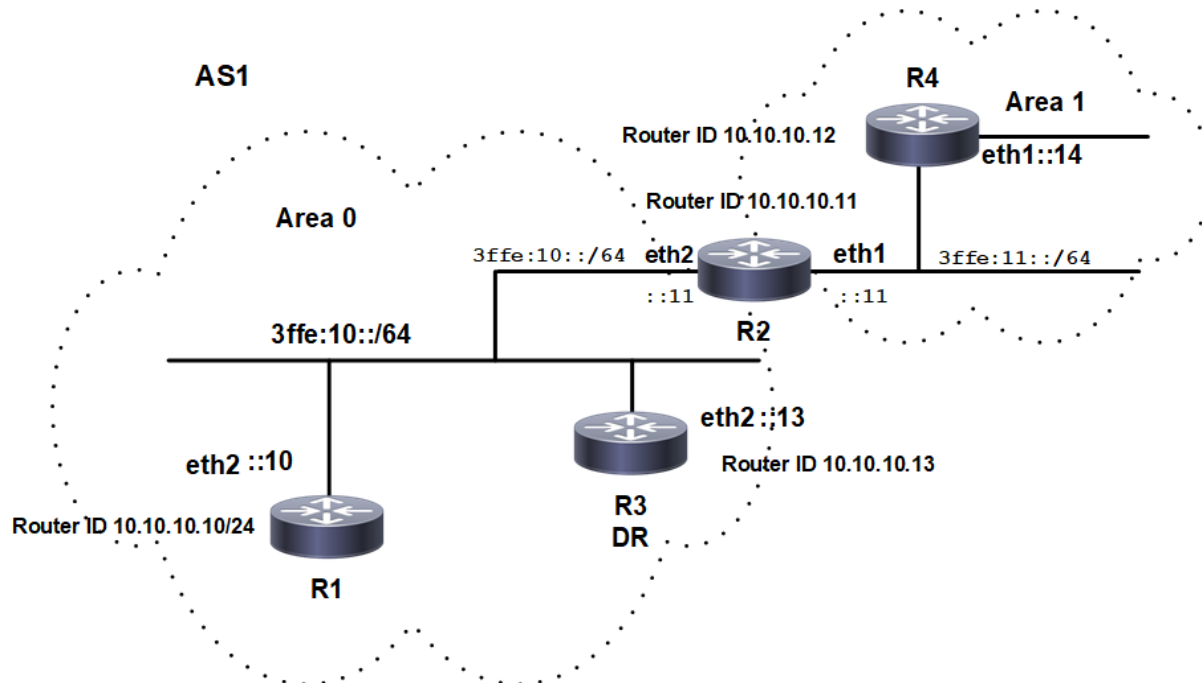
Figure 5-27: OSPFv3 Area Border Router
