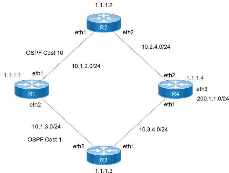
Figure 4-24: OSPF Stub Router Advertisement Topology
