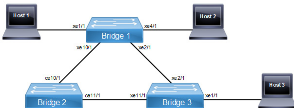
Figure 15-29: VLAN Topology
