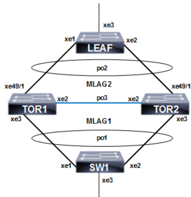
Figure 8-20: ARP ACL configuration with MC LAG
