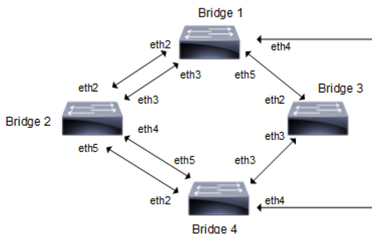
Figure 13-27: RSTP Topology
