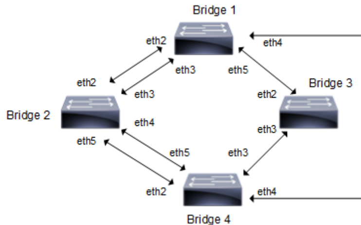
Figure 14-28: STP Topology
