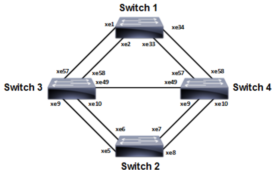
Figure 8-18: MLAG Topology
