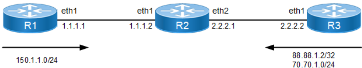
Figure 6-50: IS-IS Distance Topology
