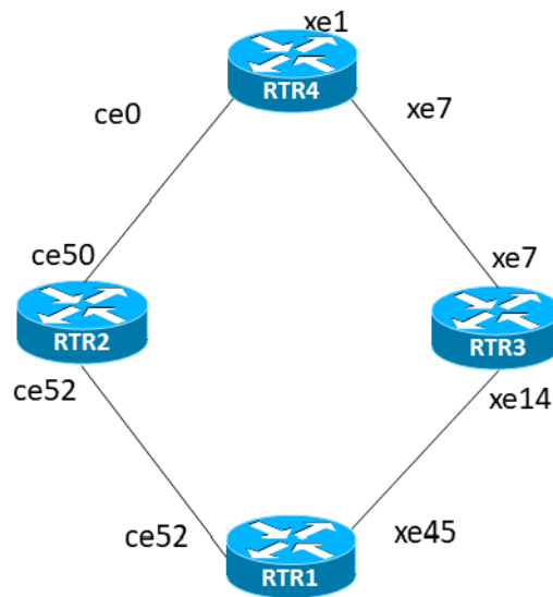
Figure 1-2: Static Route Object Tracking
