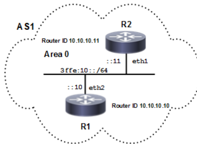
Figure 5-26: Basic OSPFv3 Topology
