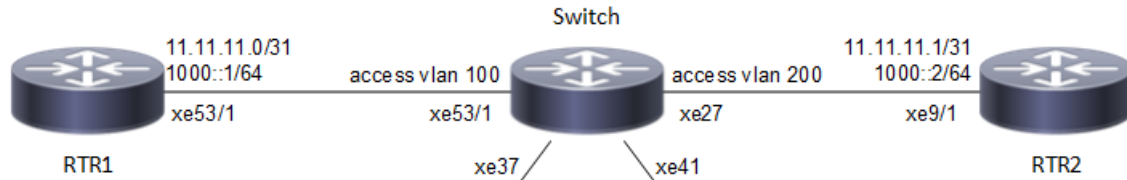
Figure P-21: BFD user-defined VRF
