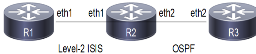
Figure 6-44: Redistribute Routes Into IS-IS
