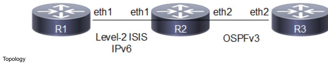
Figure 7-57: Redistribute Routes into IS-IS
