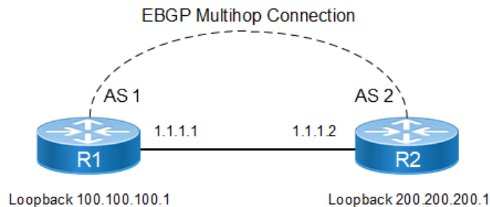
Figure 9-79: eBGP Multihop Connection
