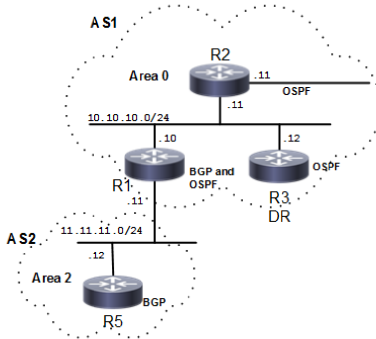
Figure 4-12: Redistribute Routes
