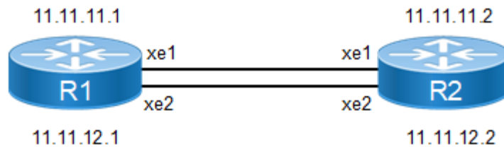
Figure 9-73: IPv4 VRF IBGP Peering
