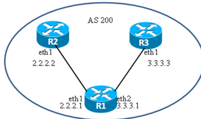
Figure 10-107: BGP Peer-Groups with IPv4 Labeled-Unicast Members
