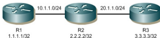
Figure P-18: Basic Topology for BFD in BGP
