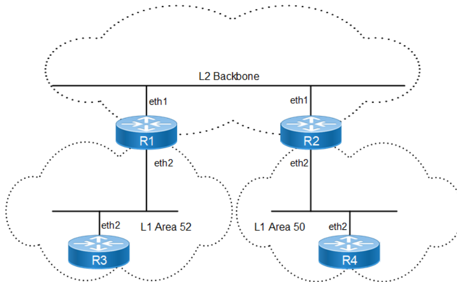
Figure 6-47: Multiple-Instance L1-L2 Area Routing
