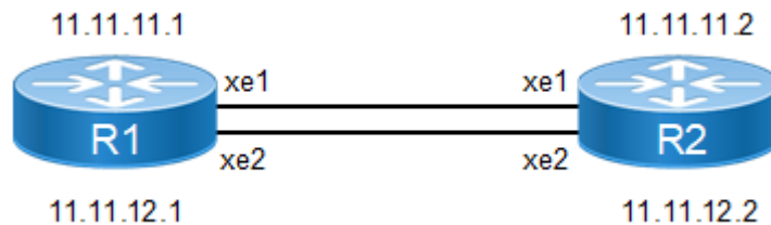
Figure 9-72: IPv4 IBGP Peering
