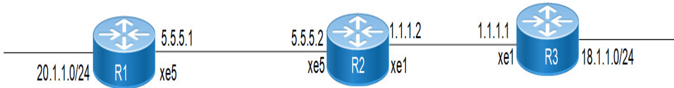
Figure 9-103: BGP Blackhole Community Attribute topology
