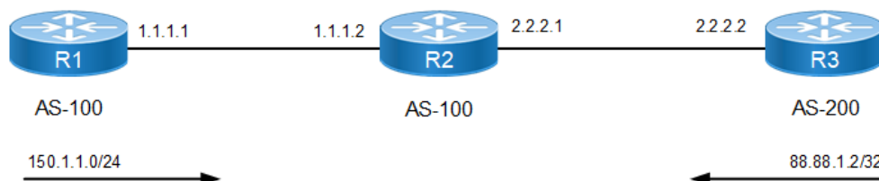
Figure 9-91: Administrative Distance for IPv4 BGP
