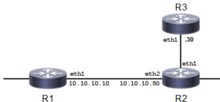
Figure 2-6: Multiple-key Topology
