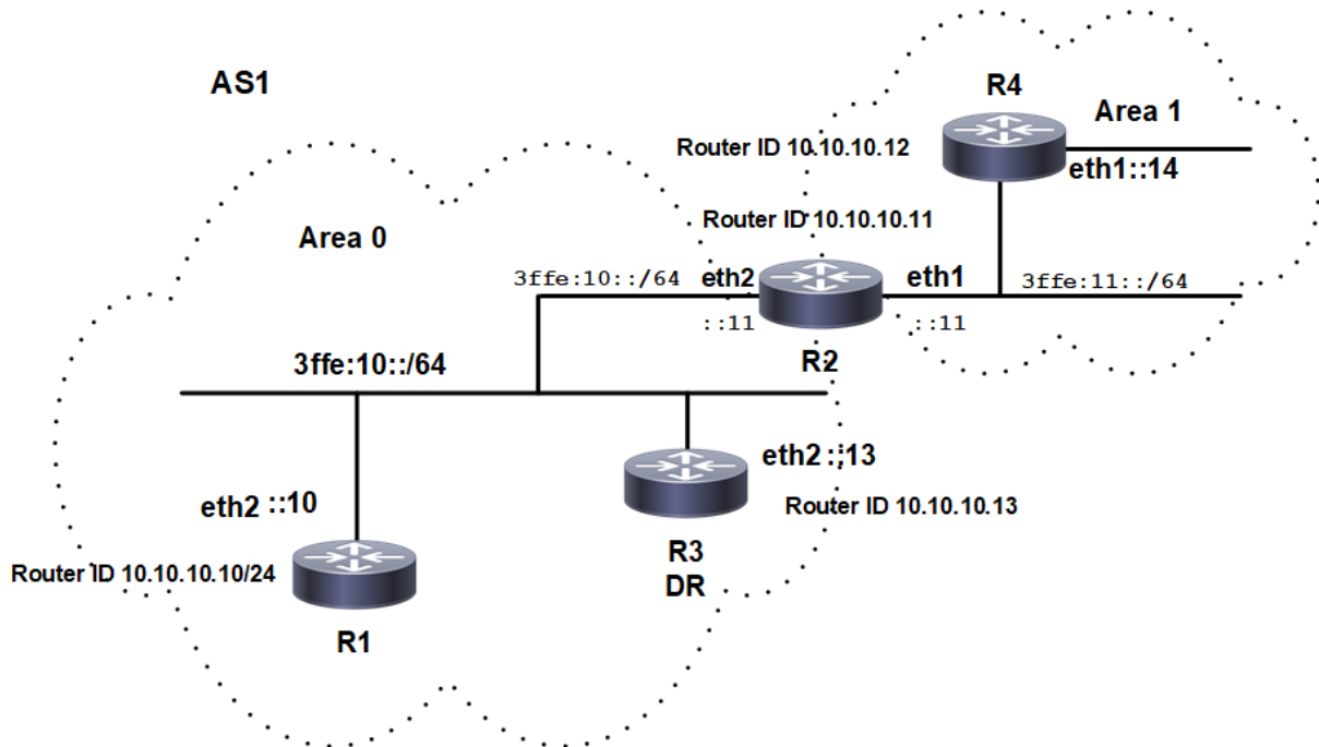
Figure 5-28: OSPFv3 Area Border Router
