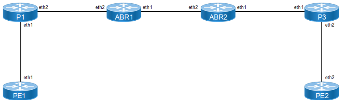
Figure 10-106: BGP Labeled unicast with Inter-AS
