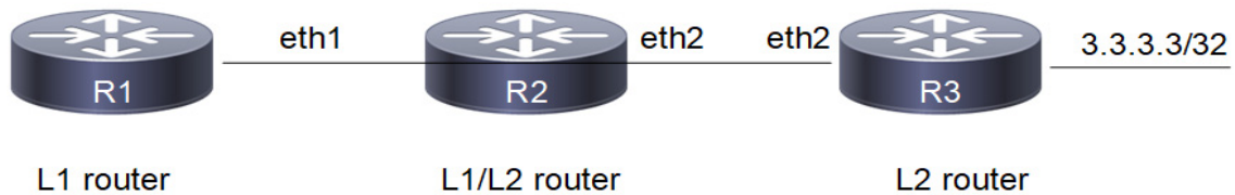
Figure 6-48: Route Leaking Topology
