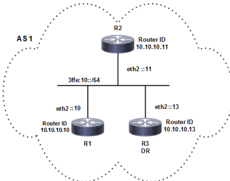
Figure 5-27: OSPFv3 Set Priority
