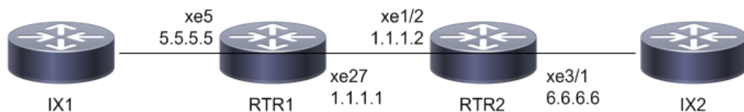
Figure 6-6: Static leaking
