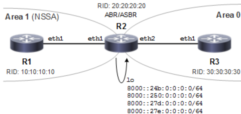
Figure 5-33: NSSA with Route Options
