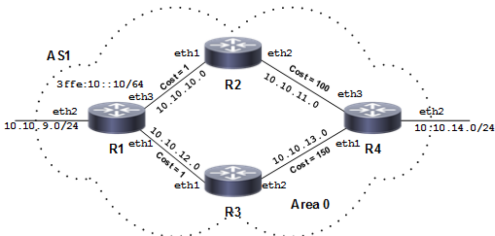
Figure 4-13: Configure Cost Topology
