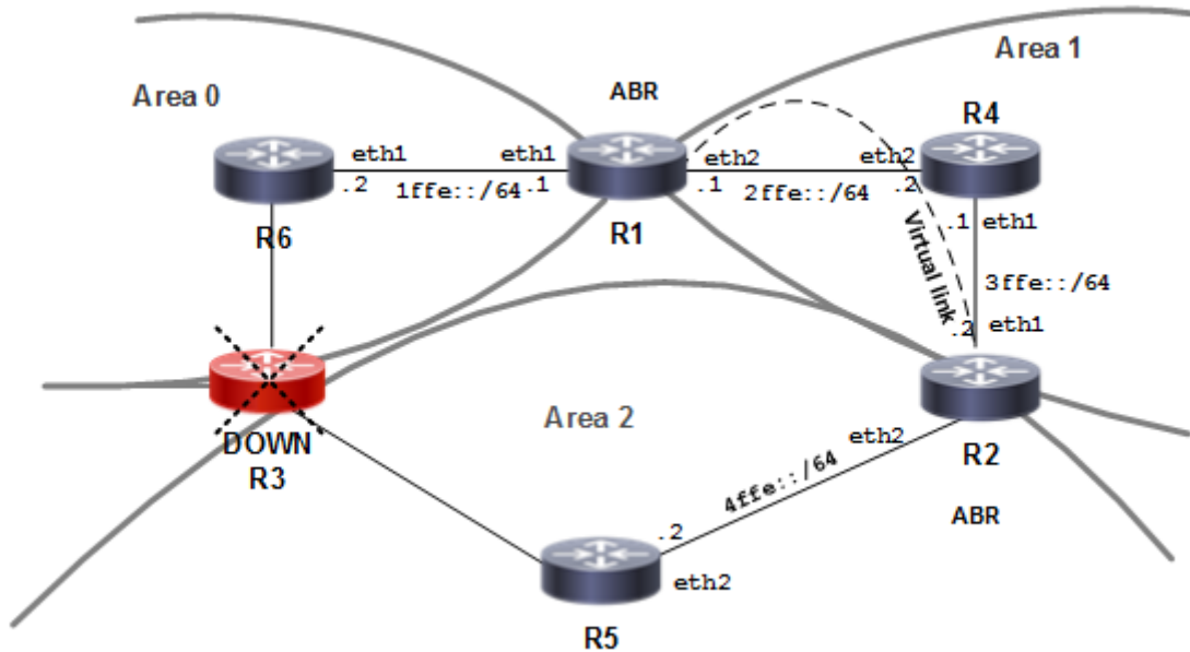
Figure 5-31: OSPFv3 Virtual Links
