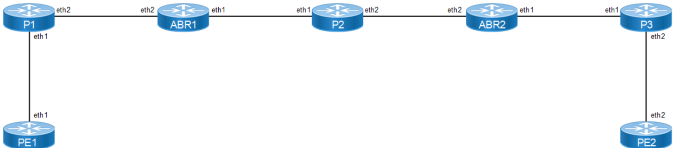
Figure 10-105: BGP_LU with MPLS
