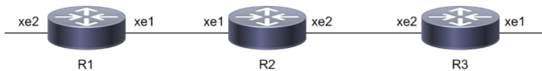
Figure 12-1: Static route discard topology
