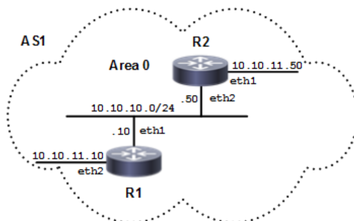
Figure 4-16: OSPF Authentication Topology
