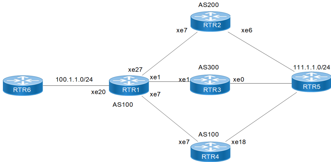
Figure 9-96: Multipath eIBGP topology
