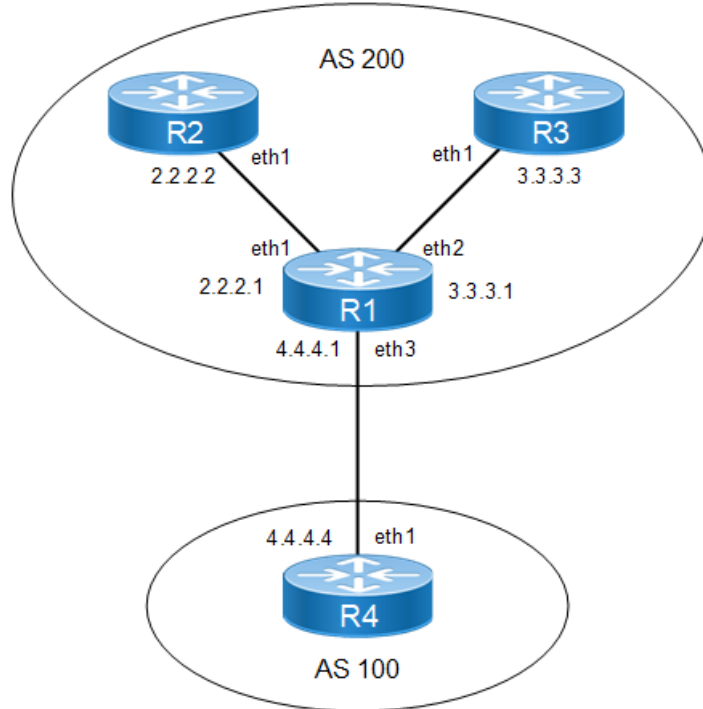
Figure 9-80: BGP Peer Groups with IPv4 Unicast Members
