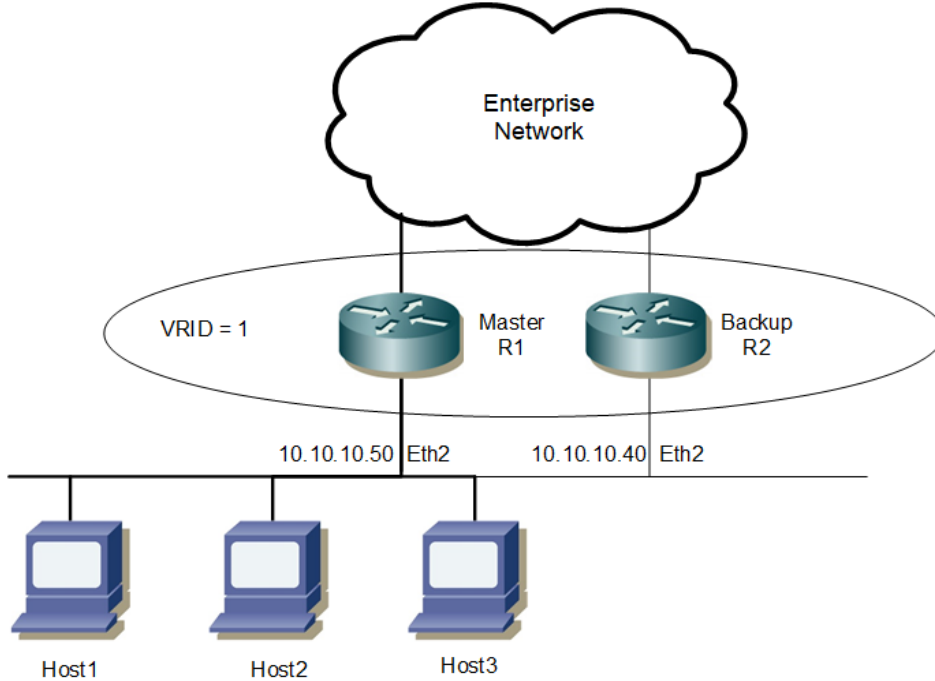
Figure 1-11: VRRP with One Virtual Router
