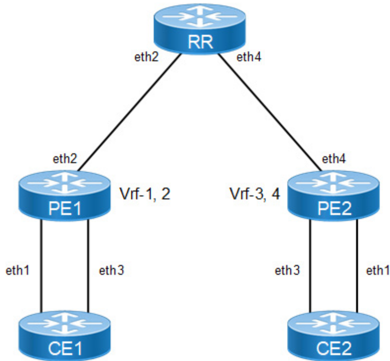
Figure 9-99: Route-target Filter Topology
